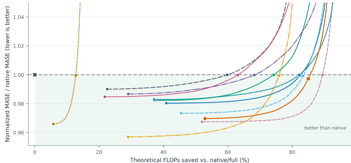
Normalized oracle Pareto frontiers of TSFMs for GiftEval
