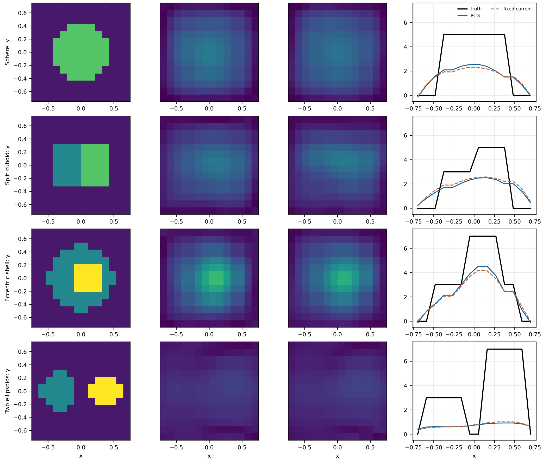
Analytic truth sampled
