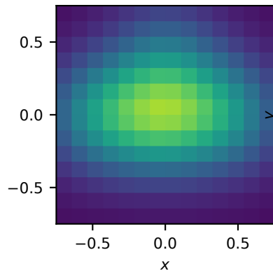
Contact / Gaussian 14^3 grid; z = 0.054
