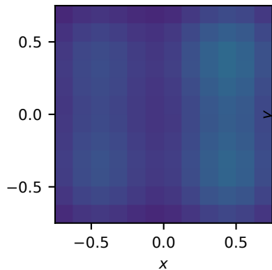
Curved / Gaussian 12^3 grid; z = -0.062
