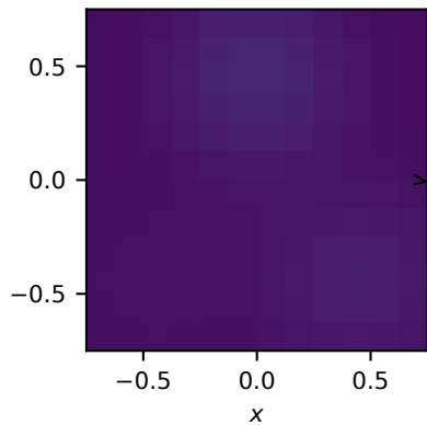
Smooth / Gaussian 12^3 grid; z = -0.062
