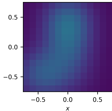
Single-pol / voxel 14^3 grid; z = 0.054
