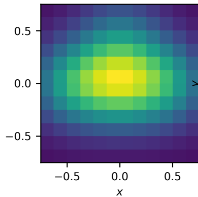
Contact / Gaussian 12^3 grid; z = -0.062
