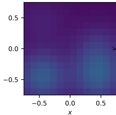
Smooth / voxel 14^3 grid; z = 0.054
