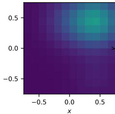
Smooth / voxel 12^3 grid; z = -0.062
