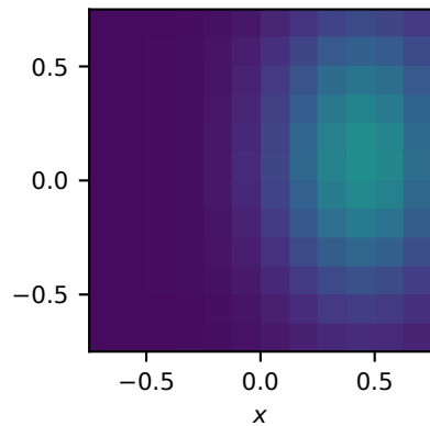
Single-pol / Gaussian 12^3 grid; z = -0.062
