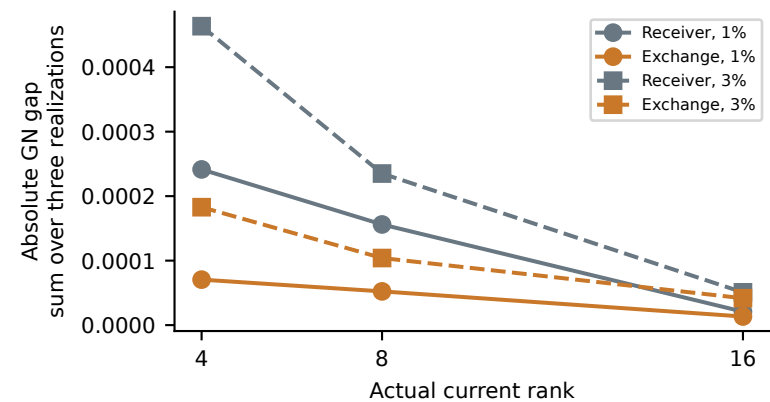
Contact, 2 inclusions, gaussian · A
