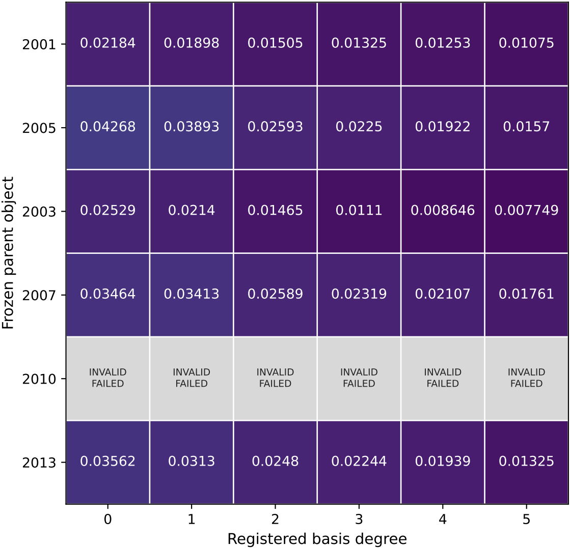
Frozen state: iteration 0
