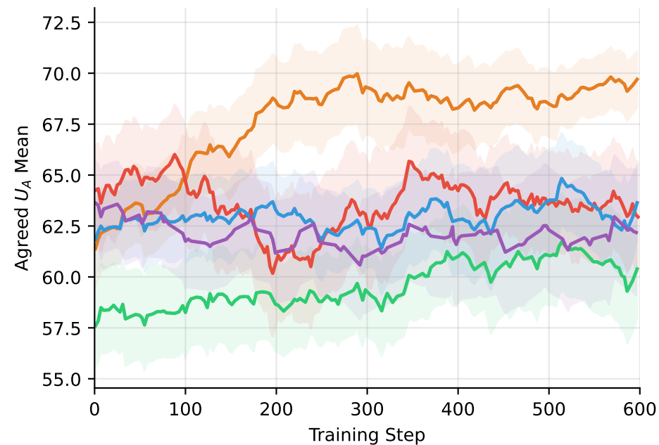
Deal Quality: Agent Payoff ( U_A )
