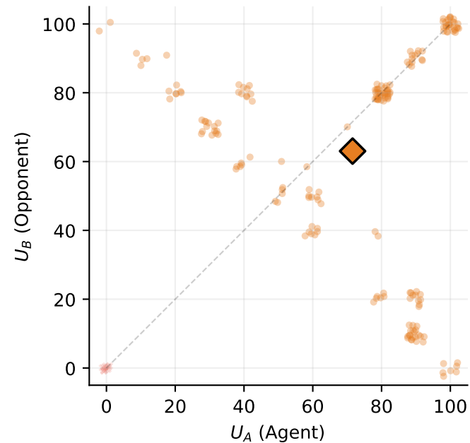
LA-GRPO Self-Only
