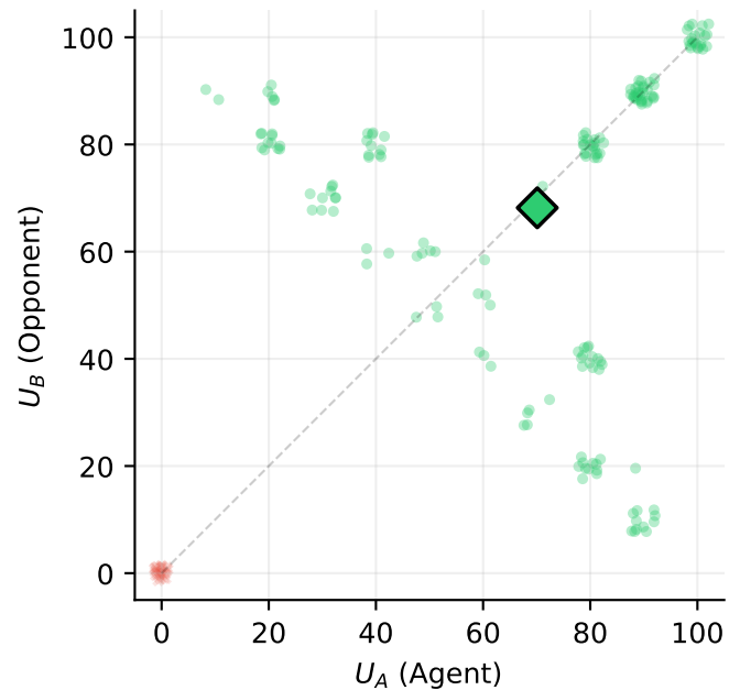
LA-GRPO Fair-Only
