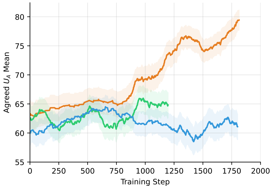
Deal Quality: Agent Payoff ( U_A )
