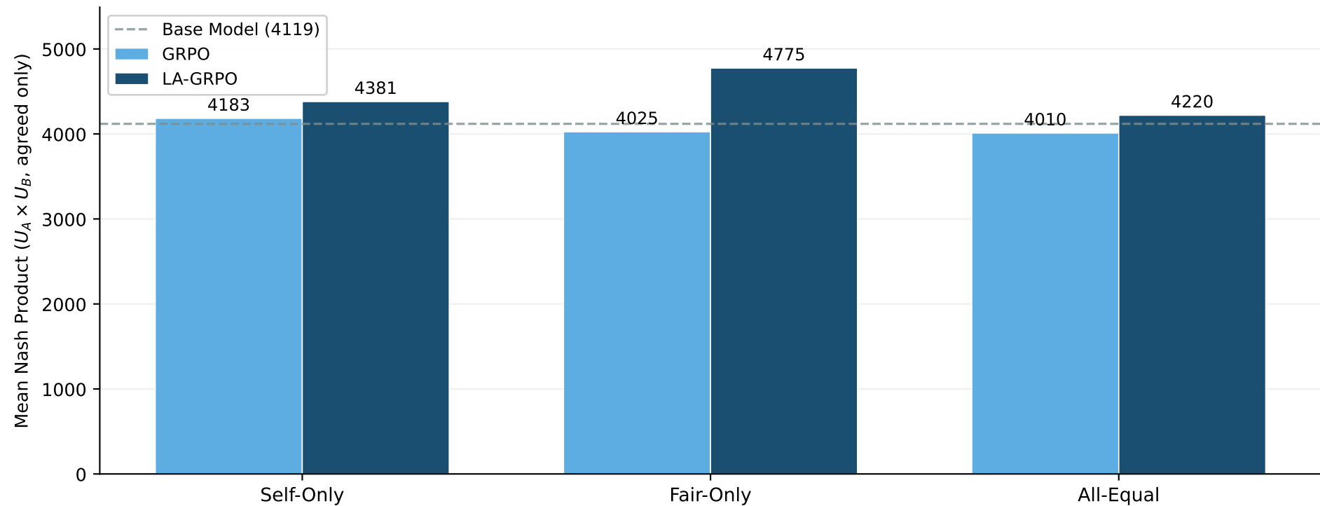
Deal Quality: Nash Product by \lambda Configuration
