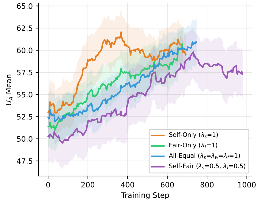
Agent Payoff ( U_A )
