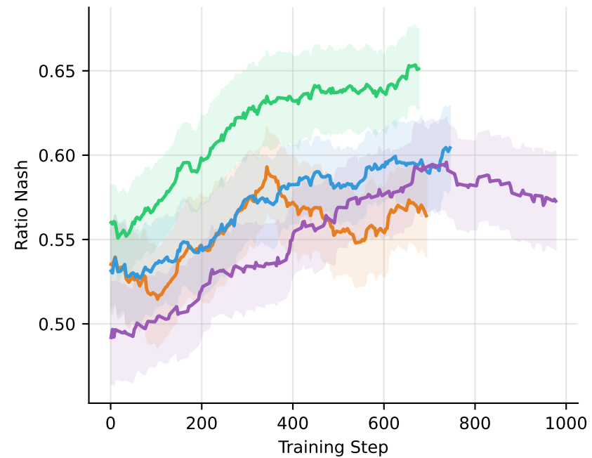
Nash Ratio (normalized)
