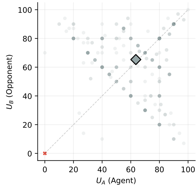
Base Model
