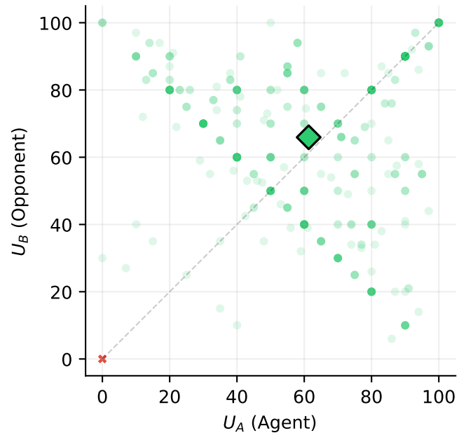
GRPO Fair-Only
