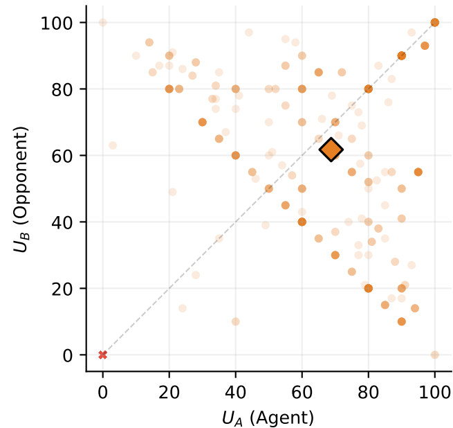
GRPO Self-Only
