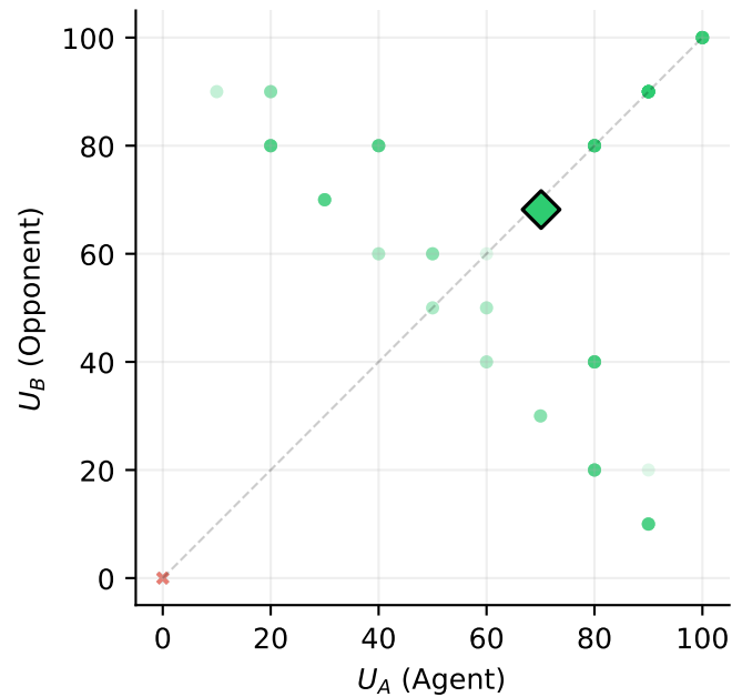
LA-GRPO Fair-Only
