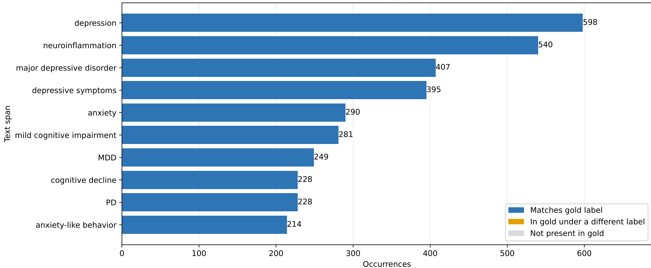
DDF entity spans
