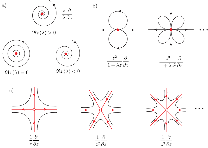
Fig. 3 forma-normal.pdf Zeros and poles of meromorphic vector fields.
