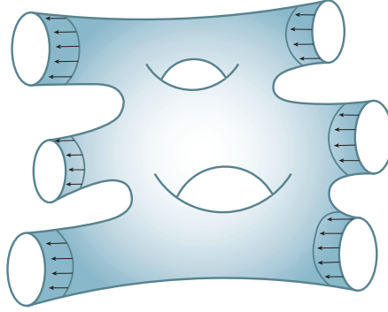
Fig. 1 figura-1.pdf The Residue Theorem as a Conservation Law.
