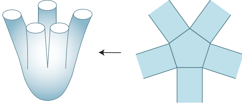
Fig. 4 figura-4.pdf Construction of a differential form with prescribed residues.
