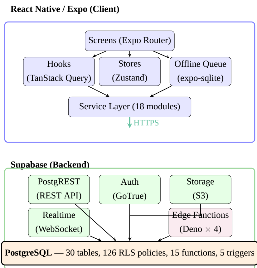
Figure 4.1: High-level system architecture. The client tier (React Native / Expo) communicates with the Supabase backend over HTTPS. Authorization is enforced at the database level by PostgreSQL Row Level Security policies.
