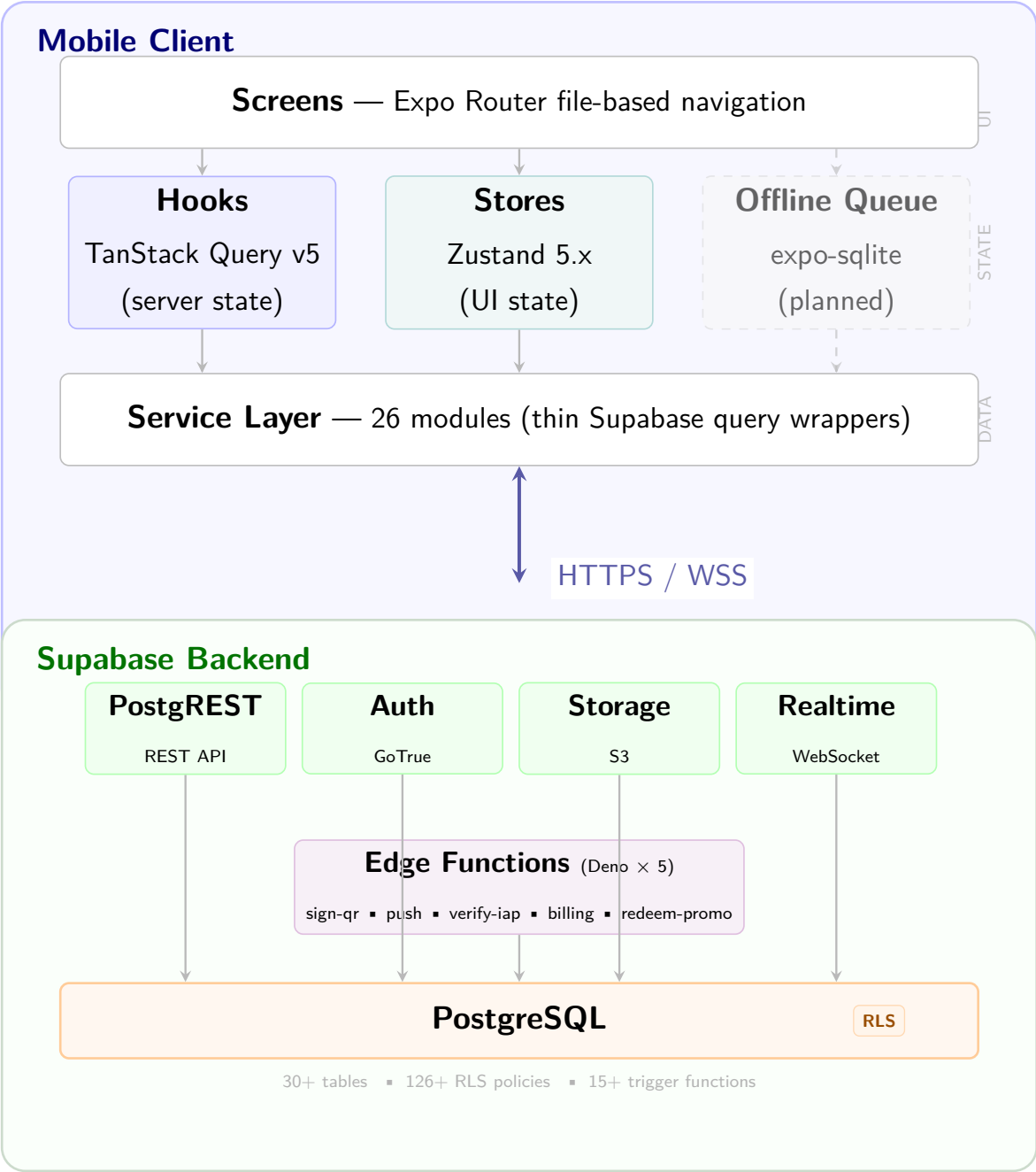
Figure 4.1: High-level system architecture. The mobile client communicates with the Supabase backend over HTTPS and WebSocket. Authorization is enforced at the database level through PostgreSQL Row Level Security (RLS) policies. Dashed elements indicate planned features.
