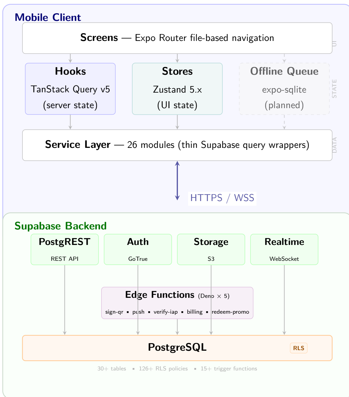
Figure 4.1: High-level system architecture. The mobile client communicates with the Supabase backend over HTTPS and WebSocket. Authorization is enforced at the database level through PostgreSQL Row Level Security (RLS) policies. Dashed elements indicate planned features.
