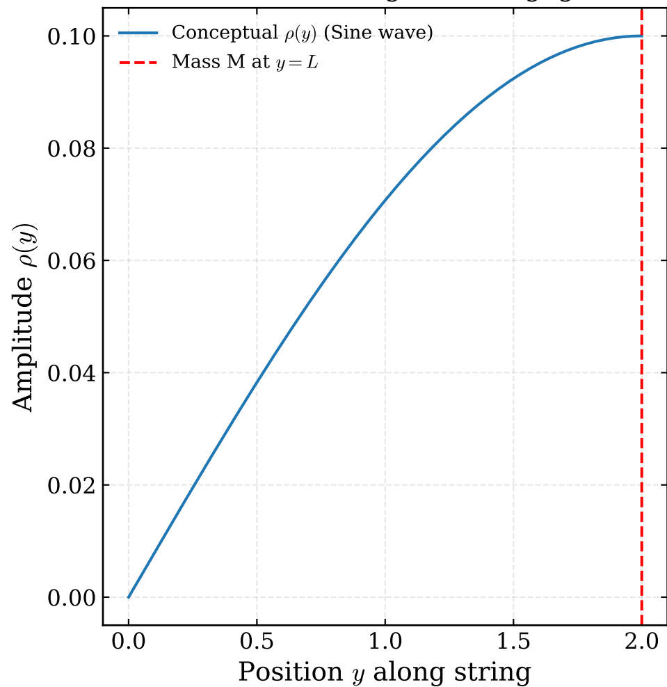
Case: m \ll M (String Mass Negligible)
