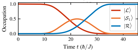
(b) Topological state occupation during transfer
