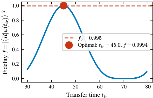
Fidelity vs transfer time ( N=2, \ell=4 )
