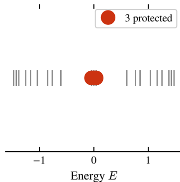
Spectrum (Third ( \sim 1/3 ))
