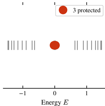
Spectrum (Center ( \sim 1/2 ))
