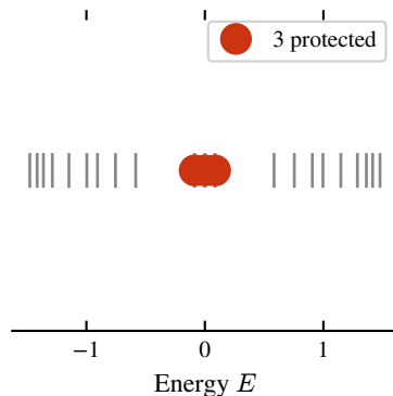
Spectrum (Quarter ( \sim 1/4 ))
