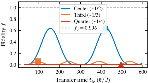
(a) Fidelity vs t_{tr} for different DW positions
