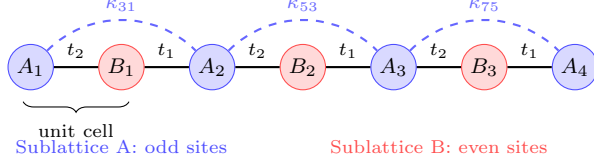
FIG. 13. Schematic of the hybrid analog-digital protocol for a chain of 2N - 1 = 7 sites. The original SSH hopping parameters t_1(t) , t_2(t) (solid lines) are supplemented by counterdiabatic NNN hoppings \kappa_{2j+1,2j-1}^{(c)} (dashed arcs) connecting neighboring sublattice A sites. The NNN terms between sublattice B sites are negligible for the zero-energy eigenstate transfer.
