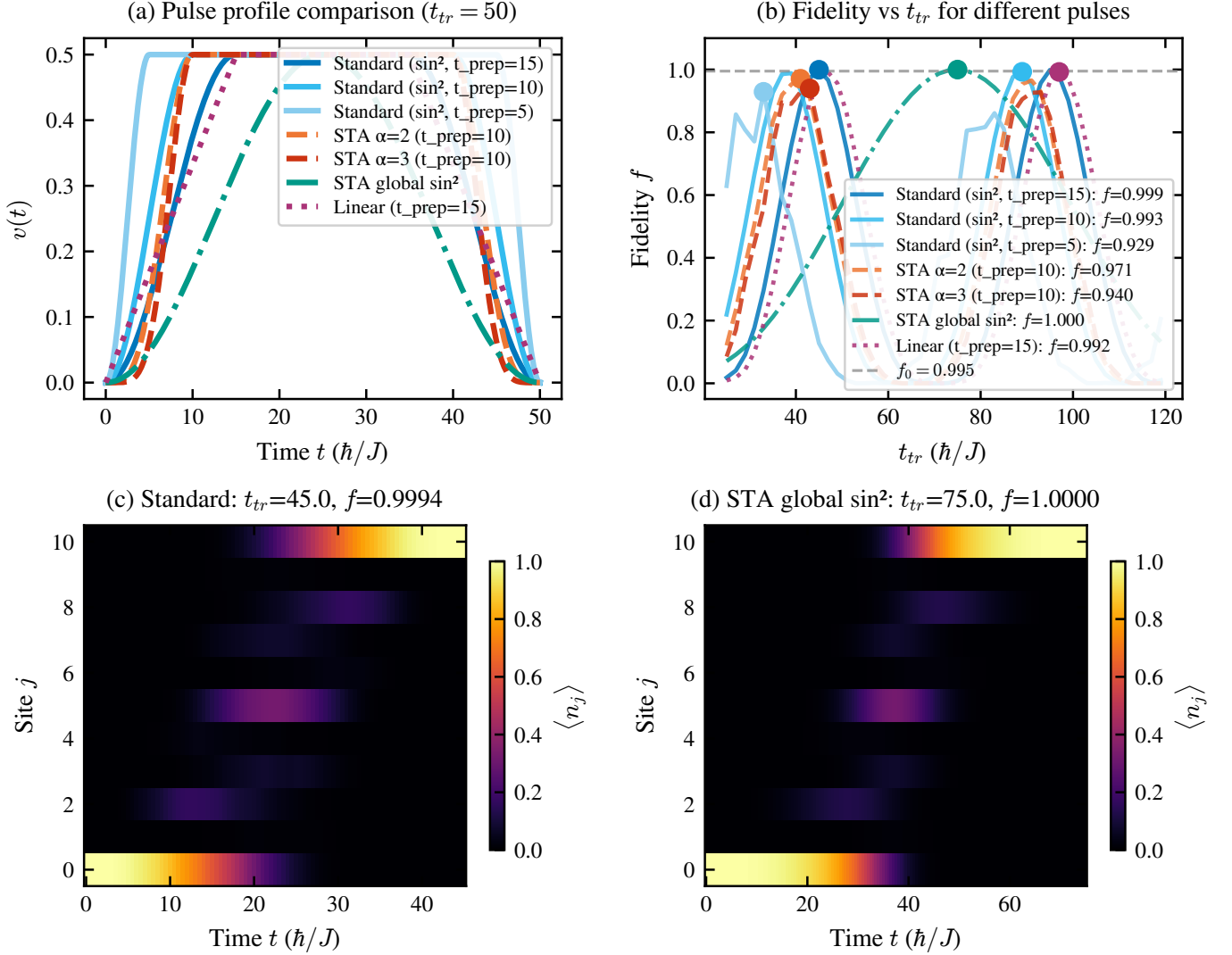
FIG. 10. Comparison of transfer fidelity vs. t_{tr} for different pulse profiles in the symmetric chain ( L=11 , \ell=4 ). The standard \sin^2 pulse with t_{\text{prep}}=15 achieves the best time-fidelity trade-off ( f=0.9994 at t_{tr}=45 ). The STA-global \sin^2 achieves the highest absolute fidelity ( f=0.99995 ) but requires t_{tr}=75 .
