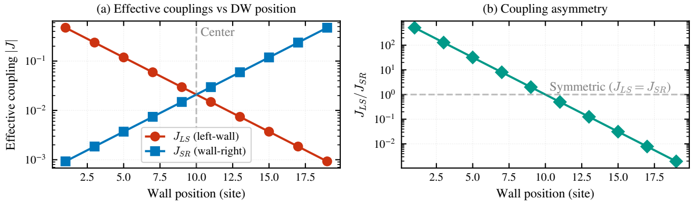
FIG. 6. Effective couplings J_{LS} (left-soliton) and J_{SR} (soliton-right) as a function of the domain wall position for L = 21 . The coupling asymmetry grows exponentially with the displacement from the chain center, consistent with Eq. (12).
