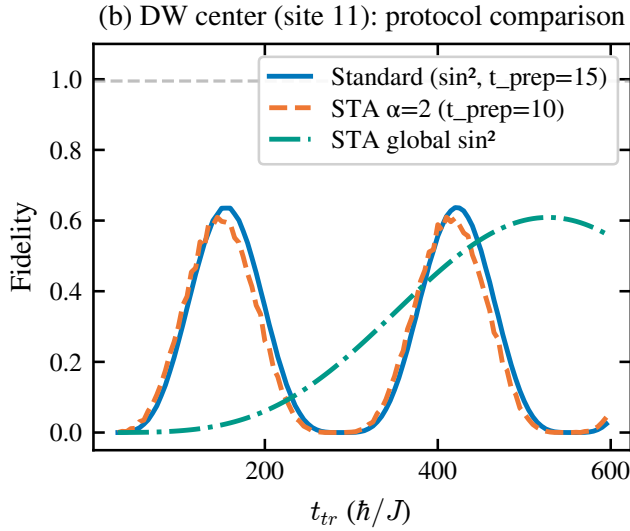
FIG. 12. Combined effect of asymmetry and STA pulses on the transfer fidelity ( L = 21 ). No pulse optimization can overcome the fundamental coupling asymmetry that limits the maximum achievable fidelity.
