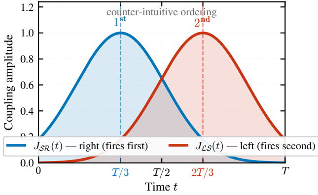
FIG. 14. (a) Counter-intuitive CTAP pulse sequence. The right-domain coupling J_{SR}(t) (blue) fires before the left-domain coupling J_{LS}(t) (red), adiabatically rotating the mixing angle \Theta(t) from 0 to \pi/2 over the transfer time T . (b) Population dynamics of the effective three-level system under the CTAP protocol ( T = 300 , \sigma = 0.18T , J_{\max} = 1 ). Starting from |\mathcal{L}\rangle (red), population is transferred to |\mathcal{R}\rangle (blue) with final fidelity f = 0.9999 . The soliton state |\mathcal{S}\rangle (gold, dashed) remains at zero throughout (lower panel, log scale)—the hallmark of dark-state transfer via the topological zero mode.
