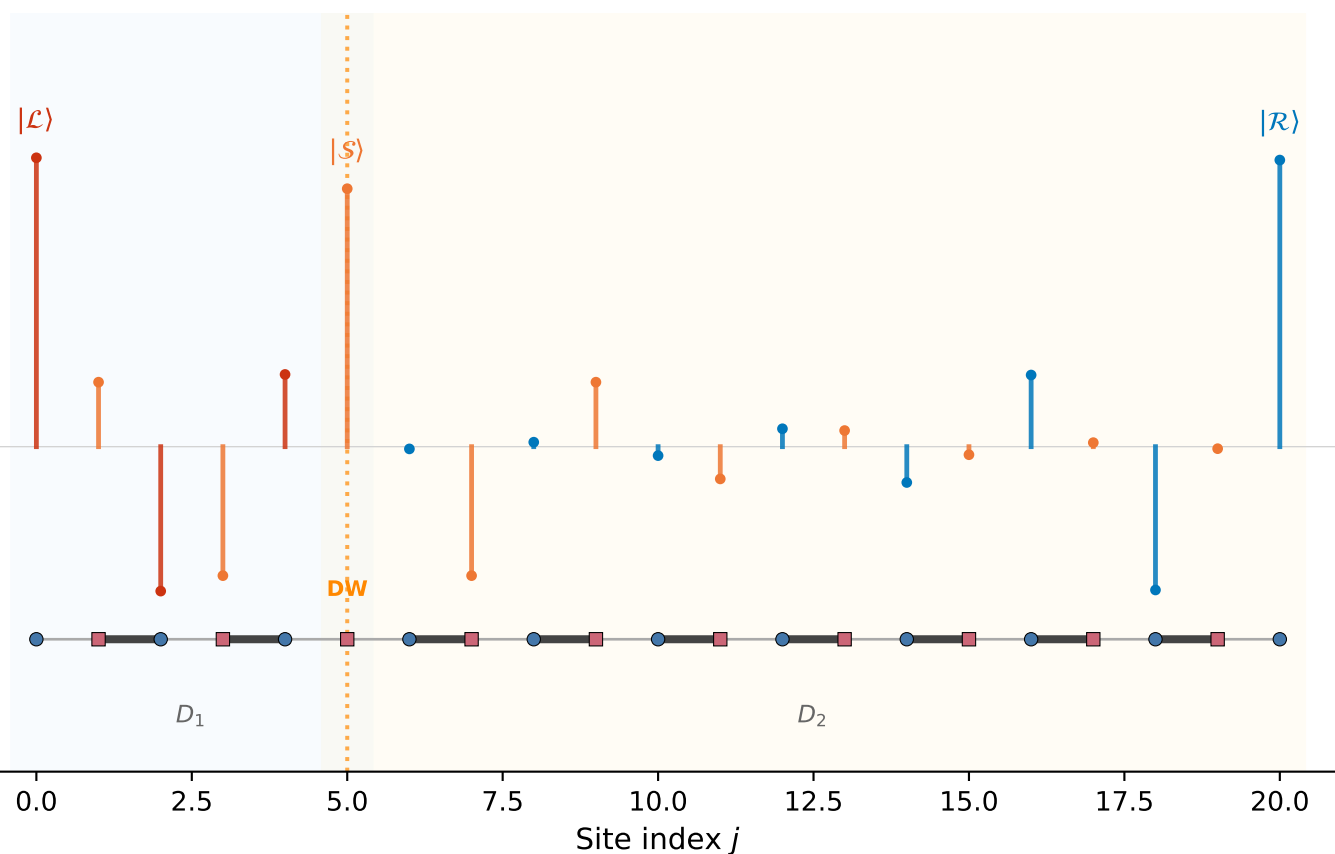
Quarter ( \sim 1/4 ): DW at site 5, L=21
