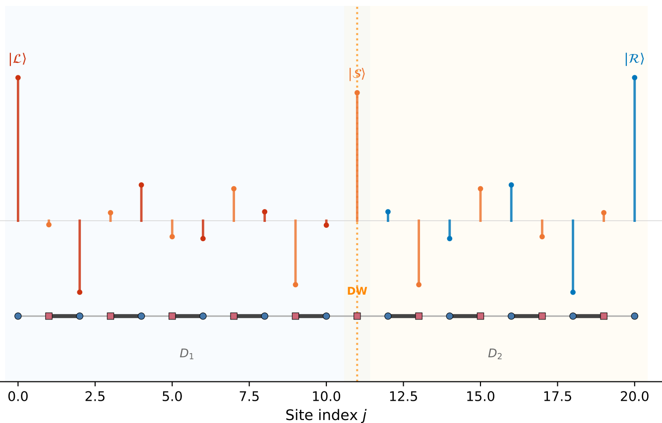
Center ( \sim 1/2 ): DW at site 11, L=21
