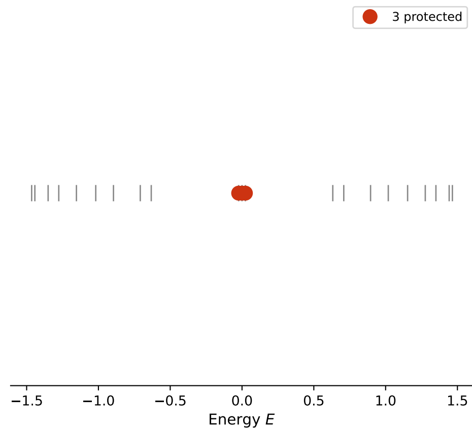
Spectrum (Center ( \sim 1/2 ))
