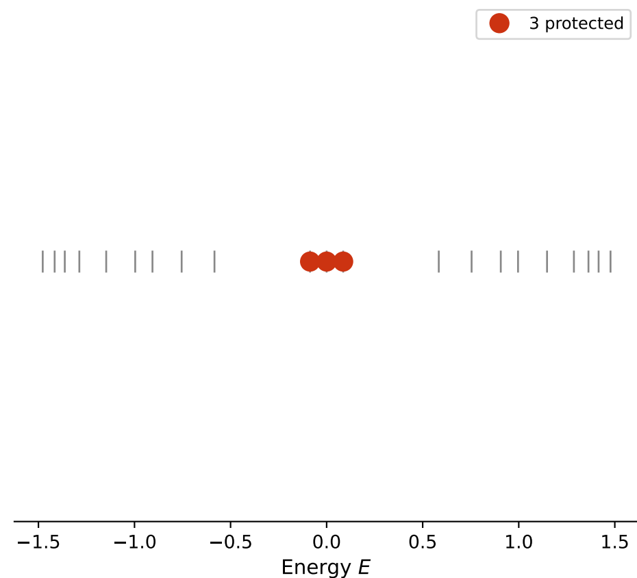
Spectrum (Quarter ( \sim 1/4 ))
