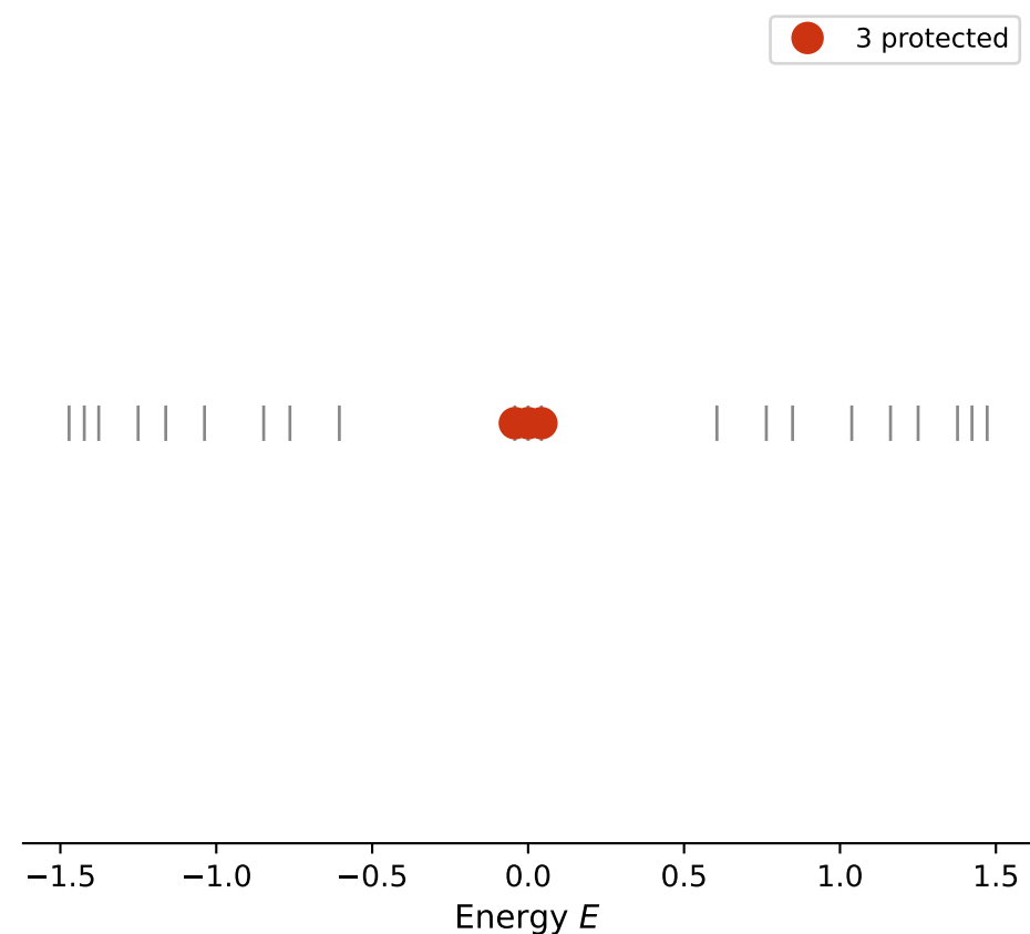
Spectrum (Third ( \sim 1/3 ))
