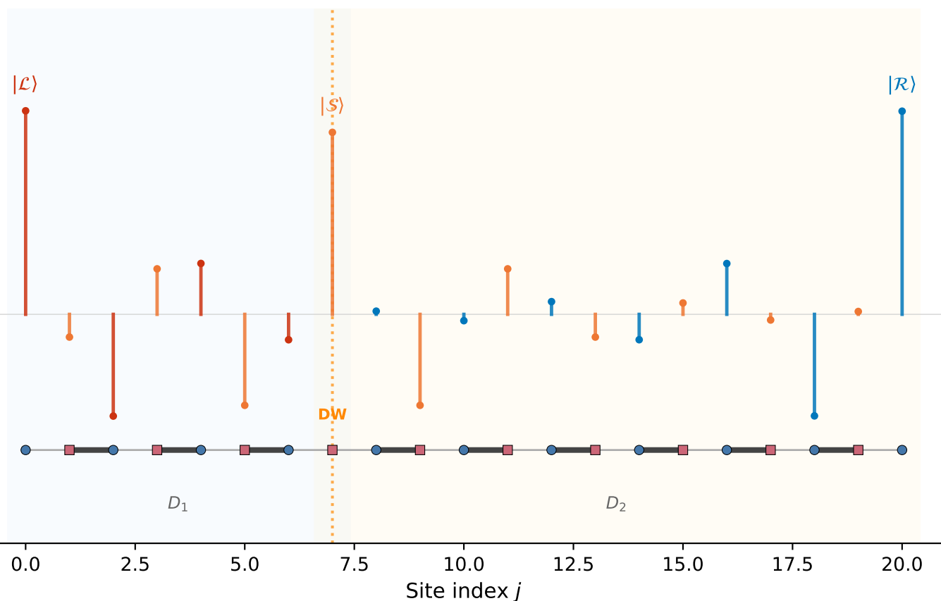
Third ( \sim 1/3 ): DW at site 7, L=21
