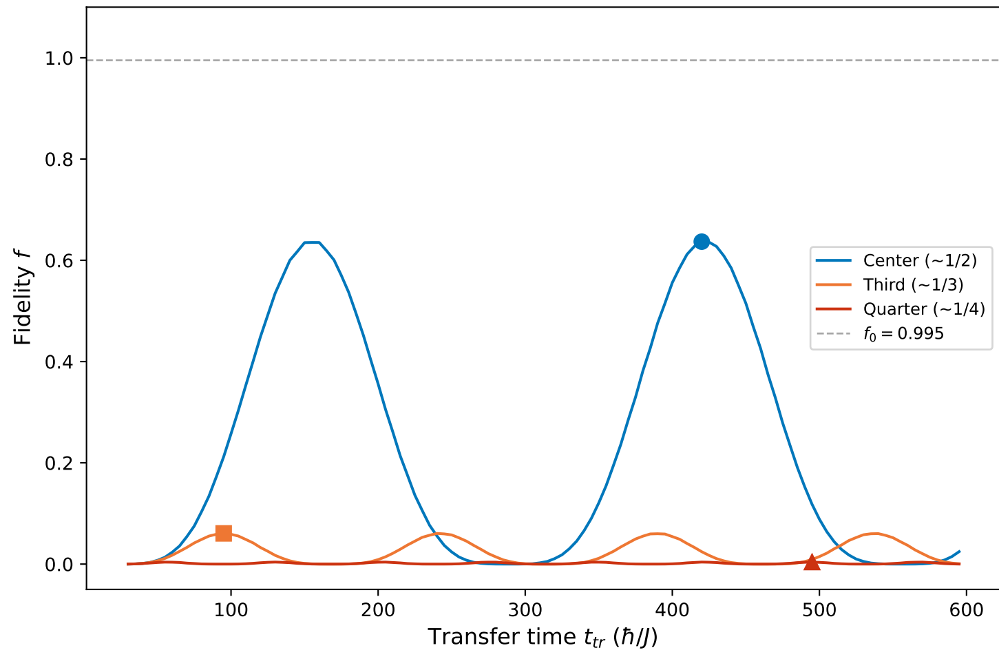
(a) Fidelity vs t_{tr} for different DW positions
