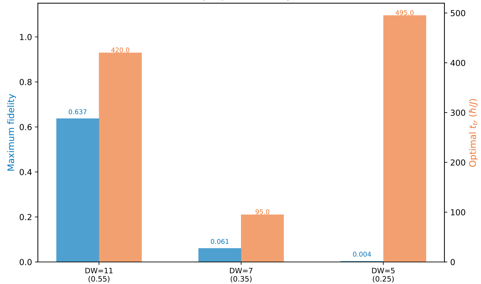
(b) Summary: optimal fidelity and time
