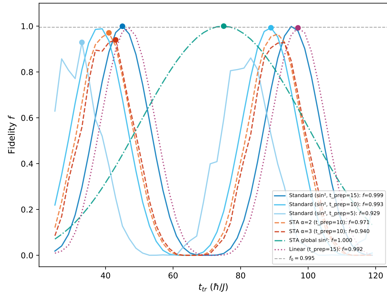
(b) Fidelity vs t_{tr} for different pulses
