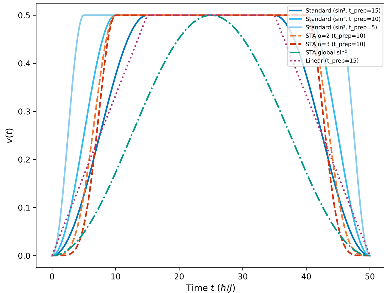
(a) Pulse profile comparison ( t_{tr} = 50 )
