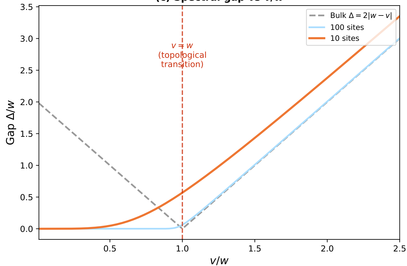
(c) Spectral gap vs v/w
