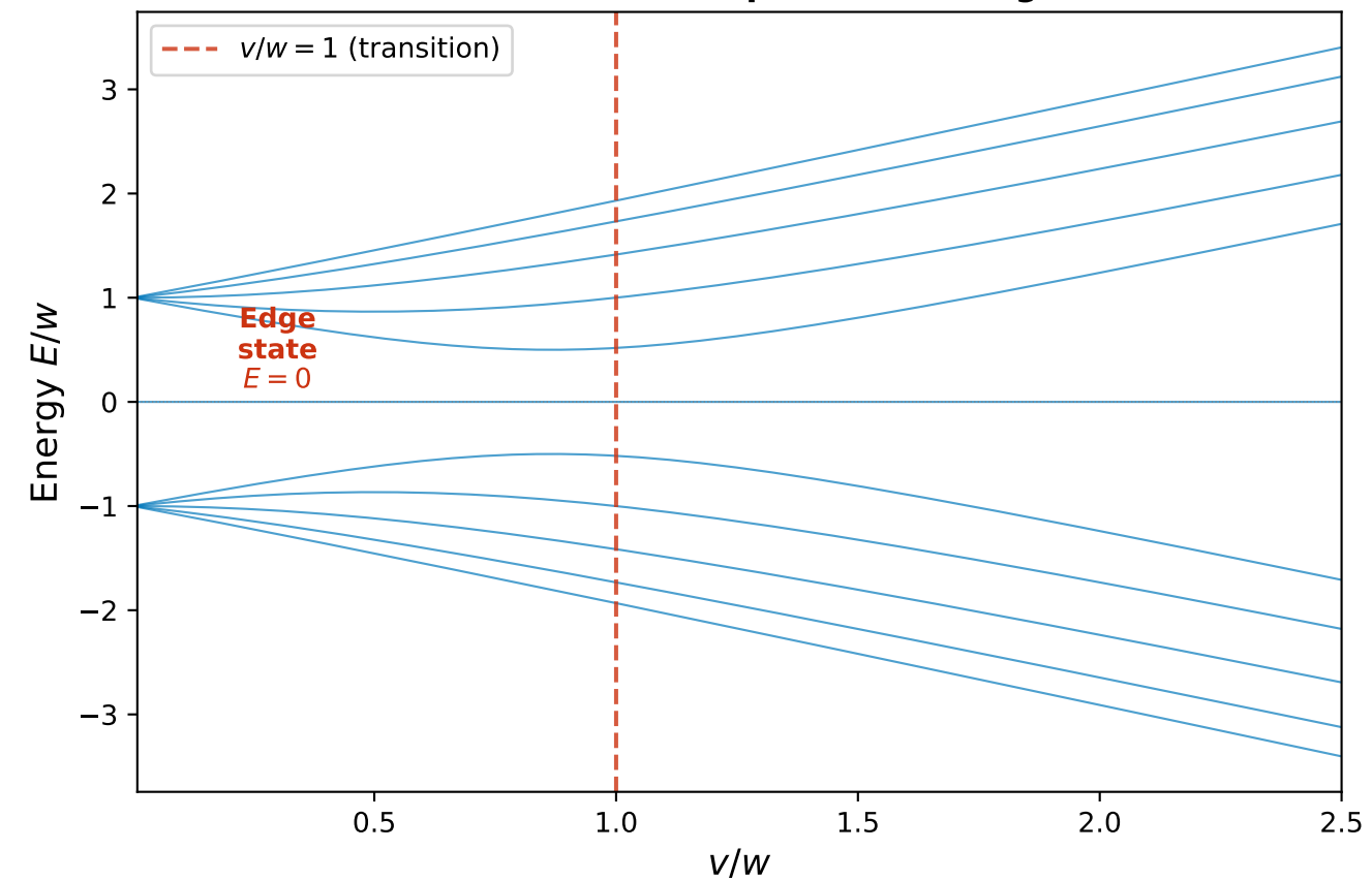
(b) Odd: 11 sites (incomplete cell \rightarrow edge state)
