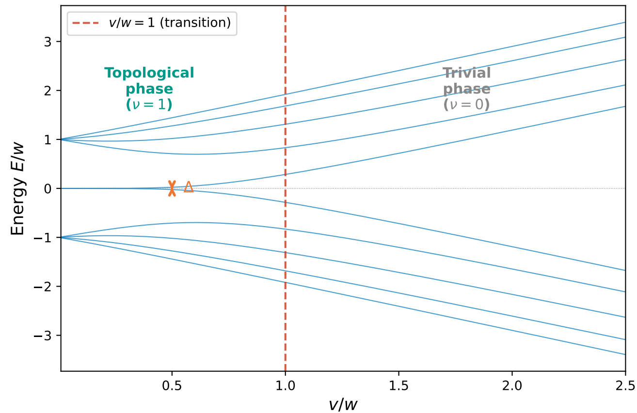
(a) Even: 10 sites (5 cells)
