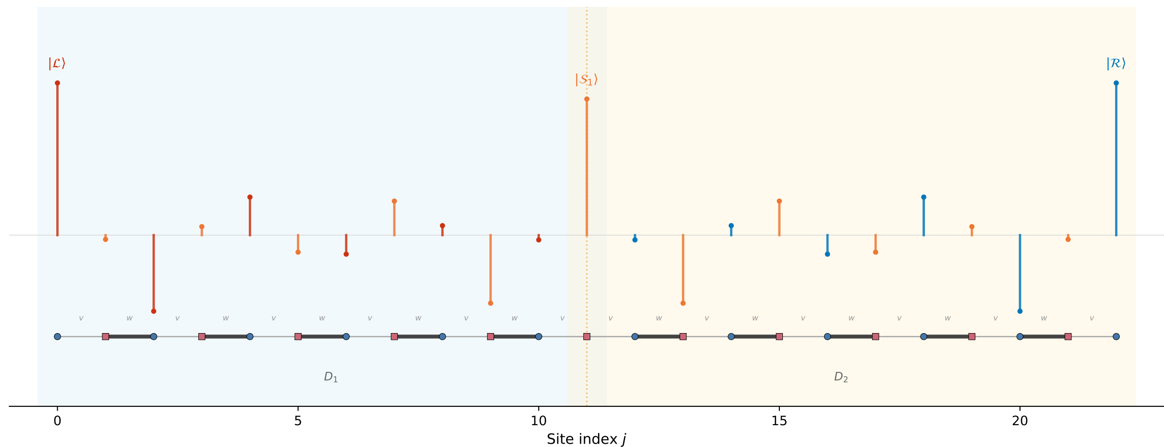
SSH chain with 1 domain wall: N = 2 , \ell = 10 , L = 23 , w = 2v = 1
