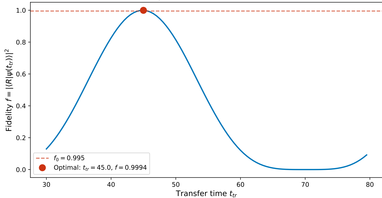
Fidelity vs transfer time ( N=2, \ell=4 )
