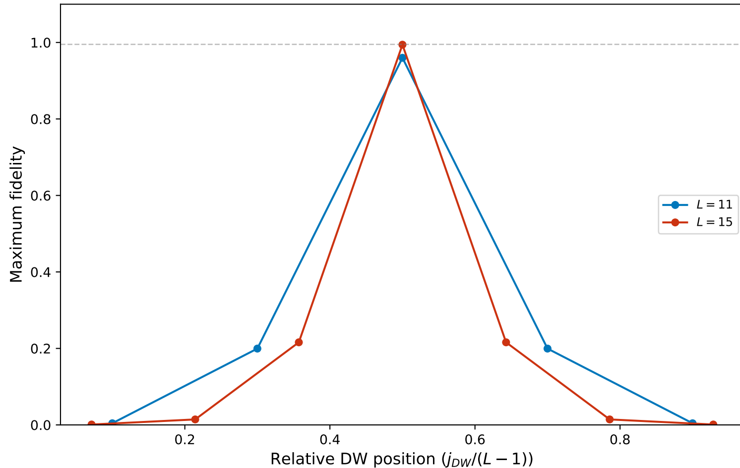
(a) Fidelity vs relative DW position
