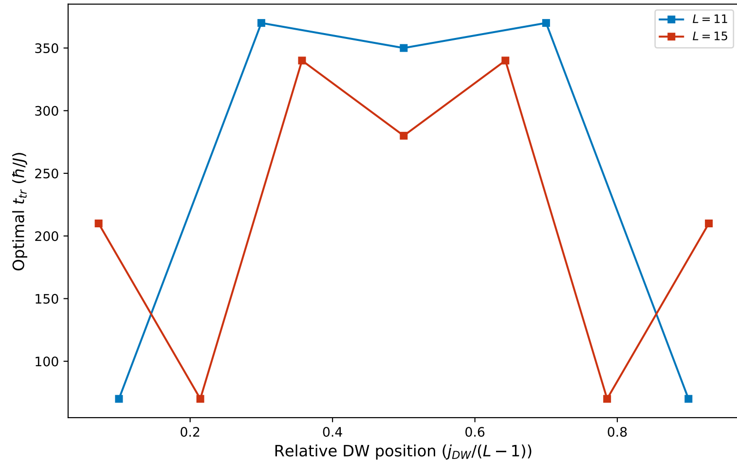
(b) Transfer time vs DW position
