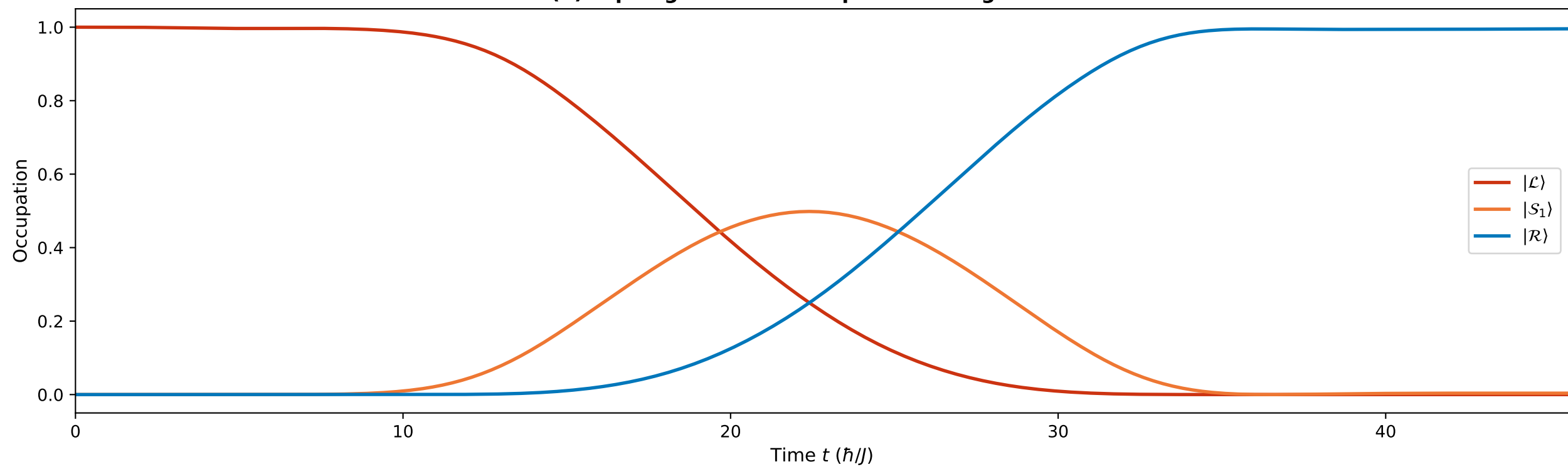
(b) Topological state occupation during transfer
