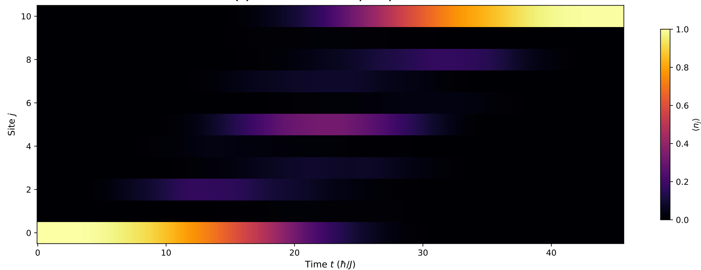
(a) Transfer L→R: N = 2, \ell = 4, L = 11
