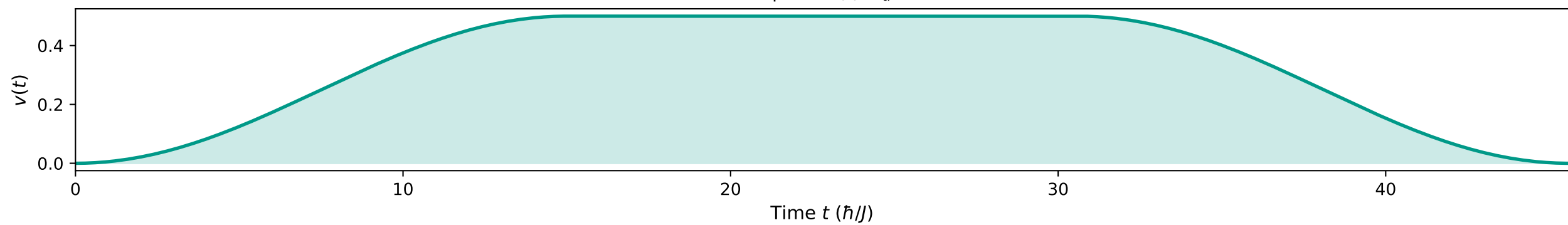
Control pulse v(t) , v_{tr} = 0.5
