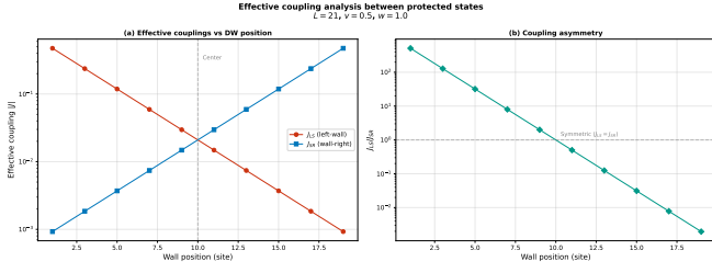
FIG. 6. Effective couplings J_{LS} (left-soliton) and J_{SR} (soliton-right) as a function of the domain wall position for L = 21 . The coupling asymmetry grows exponentially with the displacement from the chain center, consistent with Eq. (12).
