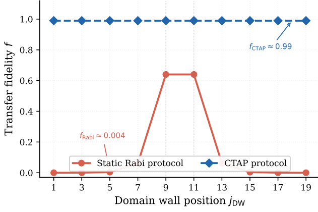
FIG. 15. Transfer fidelity versus domain wall position j_{\text{DW}} for L = 21 ( v = 0.5 , w = 1.0 ). The static Rabi protocol (red circles) peaks near f \approx 0.64 close to the chain quasi-centre and collapses exponentially to f \approx 0.004 at j_{\text{DW}} = 5 , the value computed in Sec. IV D. The CTAP protocol (blue diamonds) maintains f \approx 0.99 at all valid domain wall positions, demonstrating complete immunity to the coupling asymmetry. The shaded region represents the fidelity gain obtained by switching from the static to the dynamic protocol.
