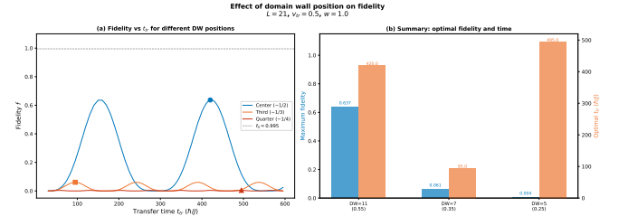
FIG. 8. Transfer fidelity as a function of t_{tr} for the three domain wall positions in the L = 21 chain. The first fidelity maximum (marked by dots) decreases exponentially with the displacement from the center.
