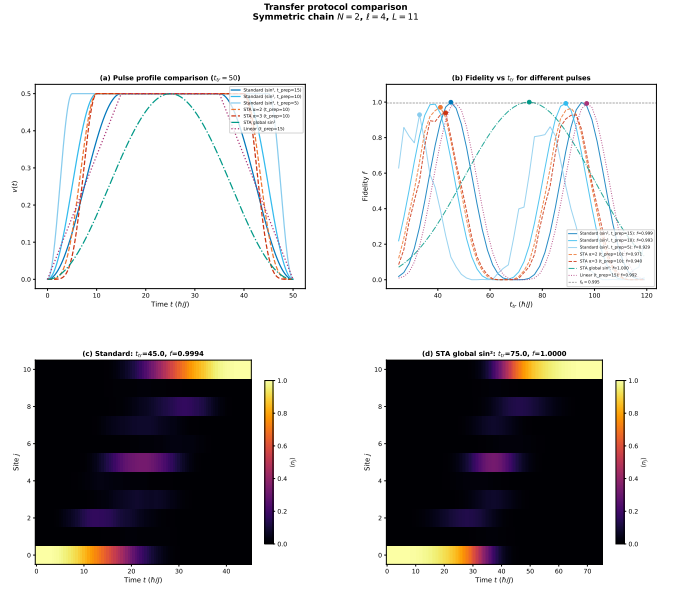
FIG. 10. Comparison of transfer fidelity vs. t_{\text{tr}} for different pulse profiles in the symmetric chain ( L = 11, \ell = 4 ). The standard \sin^2 pulse with t_{\text{prep}} = 15 achieves the best time–fidelity trade-off ( f = 0.9994 at t_{\text{tr}} = 45 ). The STA-global \sin^2 achieves the highest absolute fidelity ( f = 0.99995 ) but requires t_{\text{tr}} = 75 .
