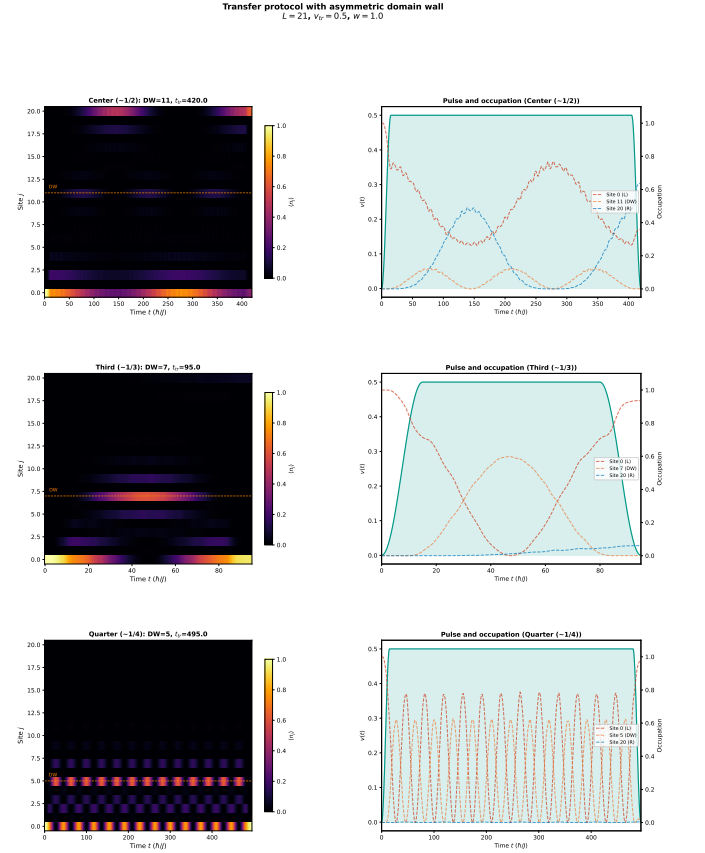
FIG. 7. Transfer dynamics for asymmetric domain wall configurations ( L = 21 ). The fidelity degrades dramatically as the domain wall moves away from the chain center.
