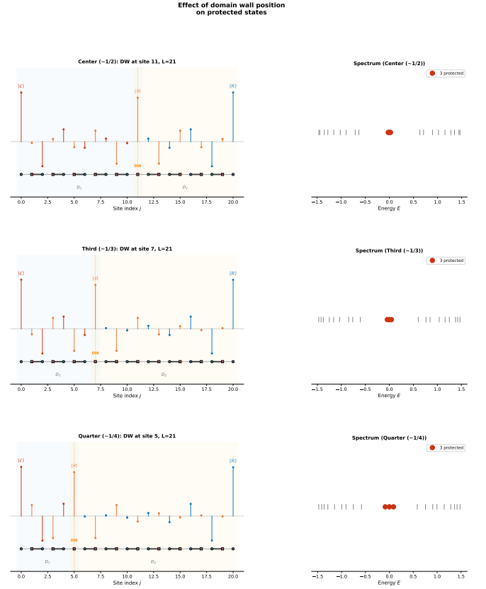
FIG. 5. Spatial profiles of the three protected states for different domain wall positions in an L = 21 chain. Top to bottom: j_{\text{DW}} = 11 (quasi-center), j_{\text{DW}} = 7 (one-third), j_{\text{DW}} = 5 (one-quarter). The exponential localization and sublattice polarization are preserved in all cases.
