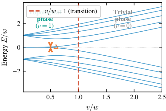
(c) Spectral gap vs v/w
