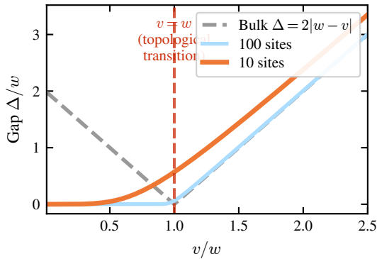
(c) Spectral gap vs v/w
