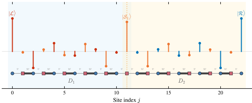
SSH chain with 1 domain wall: N=2 , \ell=10 , L=23 , w=2v=1
