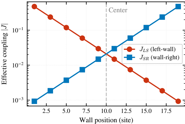
(a) Effective couplings vs DW position
