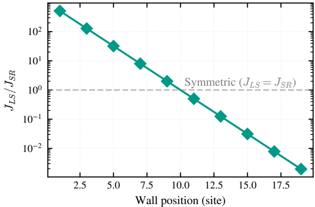
(b) Coupling asymmetry
