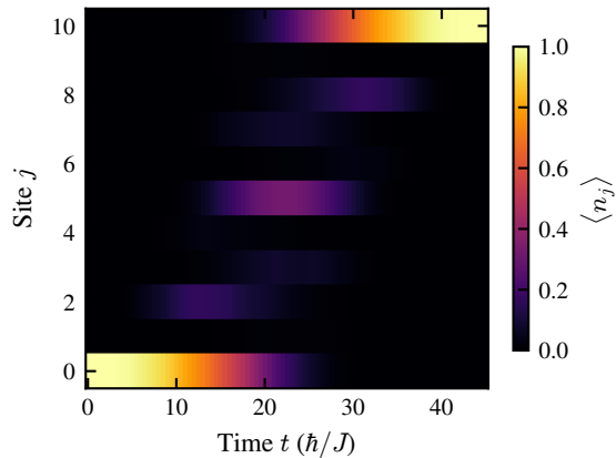
(c) Standard: t_{tr}=45.0 , f=0.9994
