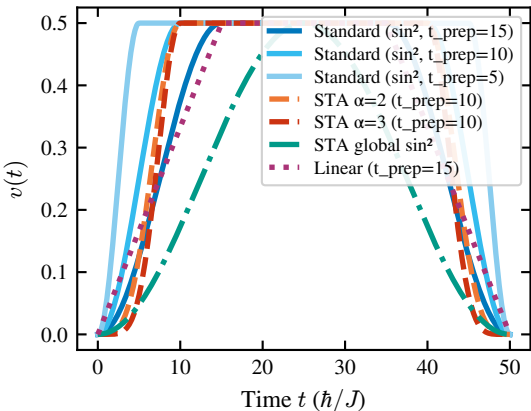
(c) Standard: t_{tr}=45.0 , f=0.9994
