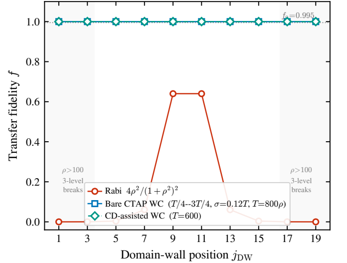
FIG. 14. Transfer fidelity versus domain-wall position j_{DW} for L = 21 ( v = 0.5 , w = 1.0 ), obtained by numerical integration of the effective three-level Hamiltonian (21). The static Rabi protocol (red circles) peaks at f \approx 0.64 near the quasi-centre and collapses to f \lesssim 0.004 for j_{DW} \leq 5 . Bare CTAP (blue squares), driven by the counter-intuitive Gaussian pulses [Eqs. (25)–(26)], sustains f > 0.99 over a broad central region and degrades only for extreme asymmetry. CD-assisted CTAP (teal diamonds) widens the high-fidelity plateau by suppressing the residual nonadiabatic error. The dotted line marks the fault-tolerance threshold f_0 = 0.995 .
