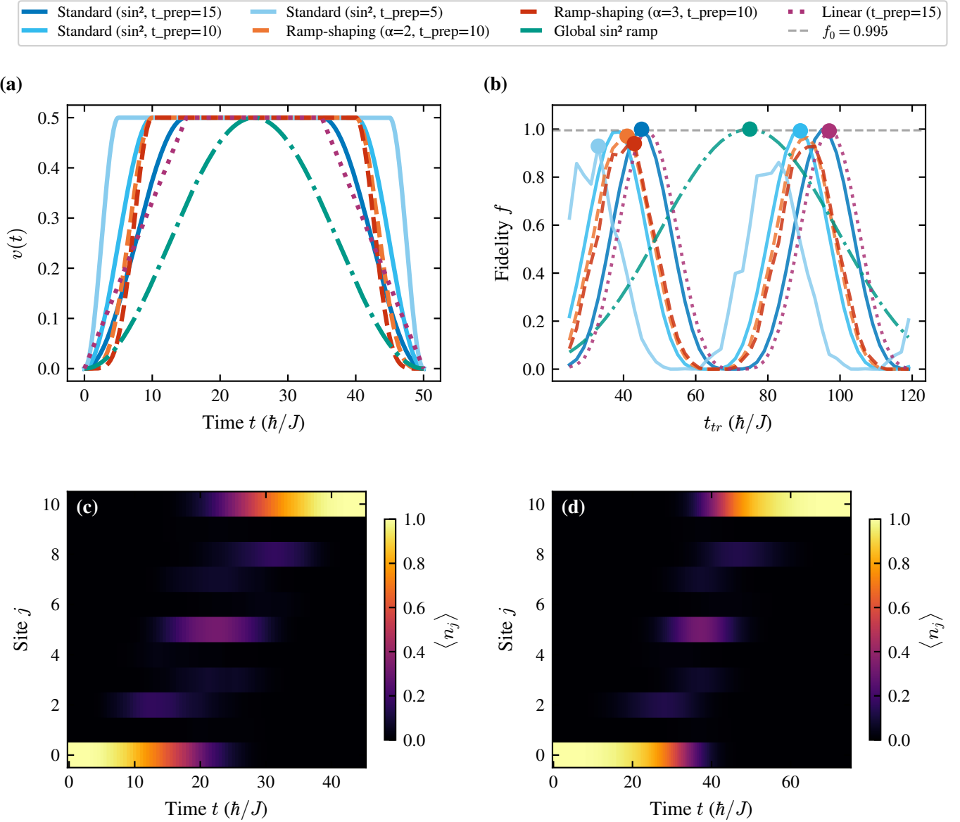
FIG. 10. Comparison of the pulse profiles for the symmetric chain ( L = 11 , \ell = 4 ). (a) The ramp shapes v(t) and (b) the resulting fidelity f vs. t_{\text{tr}} for all profiles (shared legend); dots mark each optimum. The standard \sin^2 pulse with t_{\text{prep}} = 15 (solid blue) gives the best time–fidelity trade-off ( f = 0.9994 at t_{\text{tr}} = 45 ), whereas the Global \sin^2 ramp (green dash-dot) reaches the highest absolute fidelity ( f = 0.99995 ) at the cost of t_{\text{tr}} = 75 . (c),(d) Site-resolved occupation \langle n_j \rangle vs. time for the standard \sin^2 ( t_{\text{tr}} = 45 ) and the Global \sin^2 ramp ( t_{\text{tr}} = 75 ) protocols, respectively.
