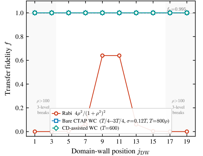
FIG. 14. Transfer fidelity versus domain-wall position j_{\text{DW}} for L = 21 ( v = 0.5 , w = 1.0 ), from numerical integration of the effective three-level Hamiltonian (21). The static Rabi protocol (red) peaks at f \approx 0.64 near the quasi-centre and collapses to f \lesssim 0.004 for j_{\text{DW}} \leq 5 . With well-conditioned pulses [Eqs. (25)–(26); peaks at T/4 and 3T/4 , \sigma = 0.12T , T = 800\rho ], bare CTAP (blue) and CD-assisted CTAP (teal) both sustain f \gtrsim 0.99 at every position where the three-level description holds, and coincide because the counterdiabatic term changes the transfer time , not the fidelity. Shaded bands ( j_{\text{DW}} \in \{1, 3, 17, 19\} , \rho \gtrsim 10^2 ) mark where the weaker coupling closes the protected gap and the three-level model no longer represents the chain. Dotted line: high-fidelity benchmark f_0 = 0.995 .
