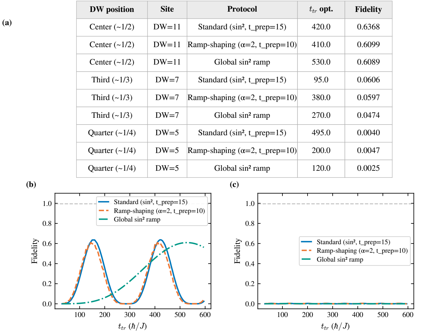
FIG. 12. Combined effect of asymmetry and ramp-shaping pulses ( L = 21 ). (a) Optimal protocol time t_{tr}^{\text{opt}} and peak fidelity for every combination of wall position ( j_{\text{DW}} = 11, 7, 5 ) and pulse profile (standard \sin^2 , Ramp-shaping ( \alpha = 2 ), Global \sin^2 ramp). (b),(c) Fidelity vs. t_{tr} for the three pulse profiles at the quasi-center ( j_{\text{DW}} = 11 , peak f \approx 0.64 ) and at a strongly asymmetric position ( j_{\text{DW}} = 5 ), respectively. At every position the three pulse variants are essentially indistinguishable and none approaches f_0 = 0.995 : pulse shaping acts only on the ramps and cannot overcome the coupling asymmetry that governs the transfer phase.
