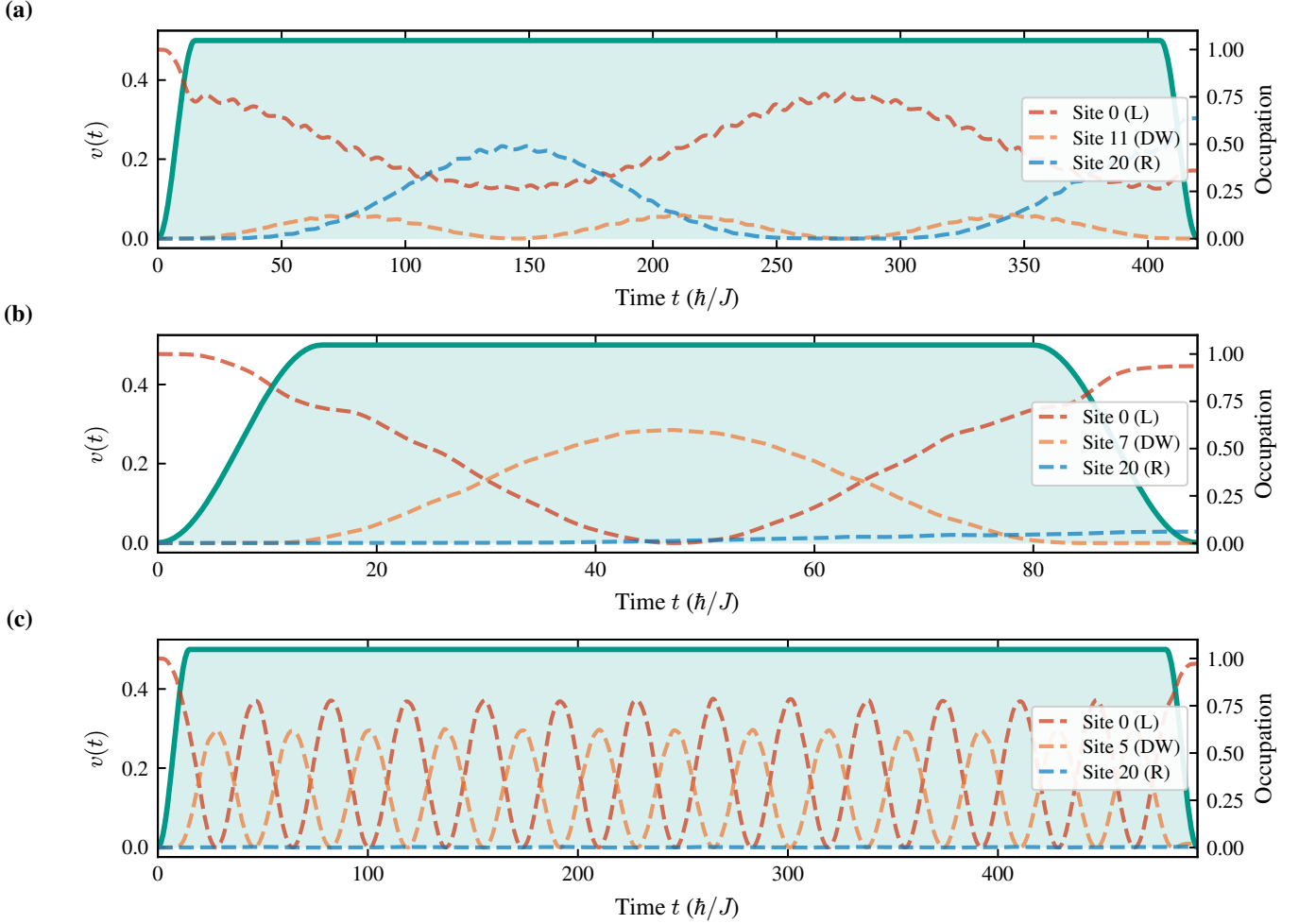
FIG. 7. Transfer dynamics for asymmetric domain wall configurations ( L = 21 ). The fidelity degrades dramatically as the domain wall moves away from the chain center.
