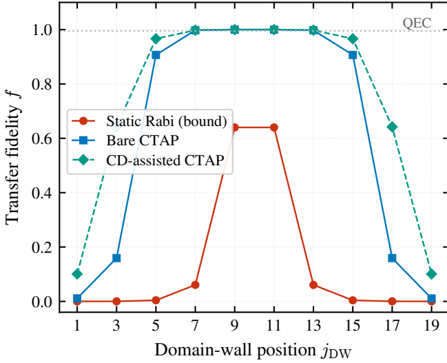
FIG. 15. Transfer fidelity versus domain-wall position j_{DW} for L = 21 ( v = 0.5 , w = 1.0 ), obtained by numerical integration of the effective three-level Hamiltonian (32). The static Rabi protocol (red circles) peaks at f \approx 0.64 near the quasi-centre and collapses to f \lesssim 0.004 for j_{DW} \leq 5 . Bare CTAP (blue squares), driven by the counter-intuitive Gaussian pulses [Eqs. (36)–(37)], sustains f > 0.99 over a broad central region and degrades only for extreme asymmetry. CD-assisted CTAP (teal diamonds) widens the high-fidelity plateau by suppressing the residual nonadiabatic error. The dotted line marks the fault-tolerance threshold f_0 = 0.995 .
