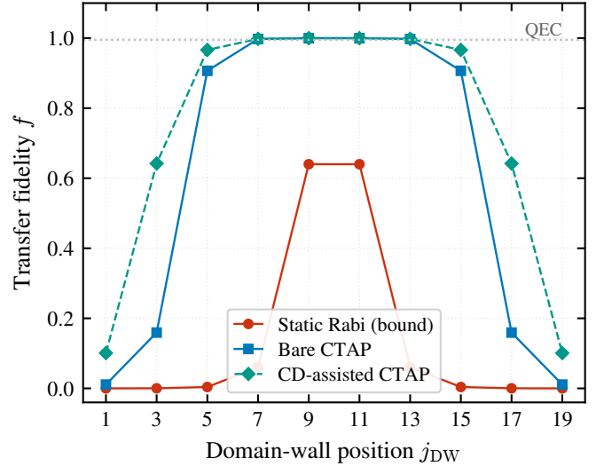
FIG. 15. Transfer fidelity versus domain-wall position j_{\text{DW}} for L = 21 ( v = 0.5 , w = 1.0 ), obtained by numerical integration of the effective three-level Hamiltonian (32). The static Rabi protocol (red circles) peaks at f \approx 0.64 near the quasi-centre and collapses to f \lesssim 0.004 for j_{\text{DW}} \leq 5 . Bare CTAP (blue squares), driven by the counter-intuitive Gaussian pulses [Eqs. (36)–(37)], sustains f > 0.99 over a broad central region and degrades only for extreme asymmetry. CD-assisted CTAP (teal diamonds) widens the high-fidelity plateau by suppressing the residual nonadiabatic error. The dotted line marks the fault-tolerance threshold f_0 = 0.995 .
