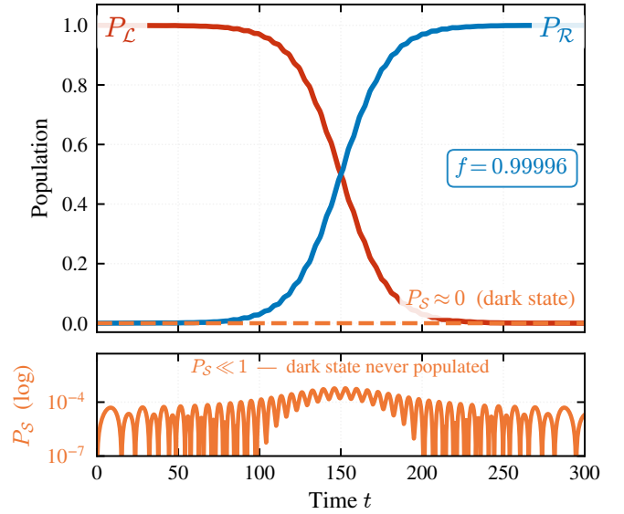
FIG. 14. (a) Counter-intuitive CTAP pulse sequence. The right-domain coupling J_{SR}(t) (blue) fires before the left-domain coupling J_{LS}(t) (red), adiabatically rotating the mixing angle \Theta(t) from 0 to \pi/2 over the transfer time T . (b) Population dynamics of the effective three-level system under the CTAP protocol ( T = 300 , \sigma = 0.18T , J_{\max} = 1 ). Starting from |\mathcal{L}\rangle (red), population is transferred to |\mathcal{R}\rangle (blue) with final fidelity f = 0.9999 . The soliton state |\mathcal{S}\rangle (gold, dashed) remains at zero throughout (lower panel, log scale)—the hallmark of dark-state transfer via the topological zero mode.
