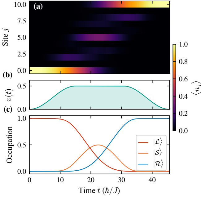
FIG. 3. Transfer protocol dynamics for the symmetric two-domain SSH chain ( L = 11 , \ell = 4 , v_{\text{tr}} = 0.5 , w = 1.0 , t_{\text{prep}} = 15 , t_{\text{tr}} = 45 ). Population is transferred from site 0 to site 10 via the topologically protected subspace, with final fidelity f = 0.999 .
