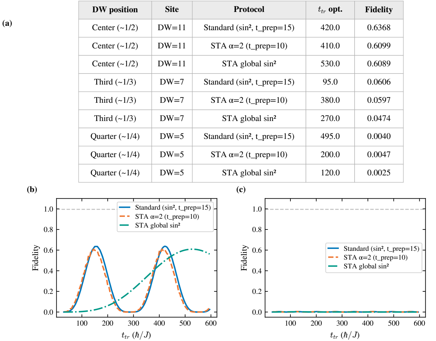
FIG. 12. Combined effect of asymmetry and STA pulses on the transfer fidelity ( L = 21 ). No pulse optimization can overcome the fundamental coupling asymmetry that limits the maximum achievable fidelity.
