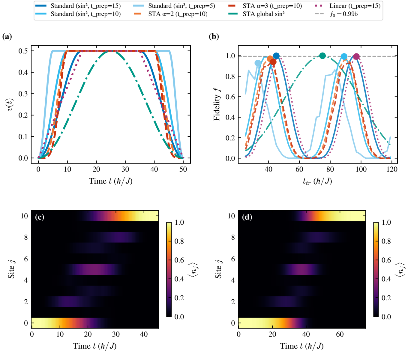
FIG. 10. Comparison of transfer fidelity vs. t_{\text{tr}} for different pulse profiles in the symmetric chain ( L = 11 , \ell = 4 ). The standard \sin^2 pulse with t_{\text{prep}} = 15 achieves the best time-fidelity trade-off ( f = 0.9994 at t_{\text{tr}} = 45 ). The STA-global \sin^2 achieves the highest absolute fidelity ( f = 0.99995 ) but requires t_{\text{tr}} = 75 .
