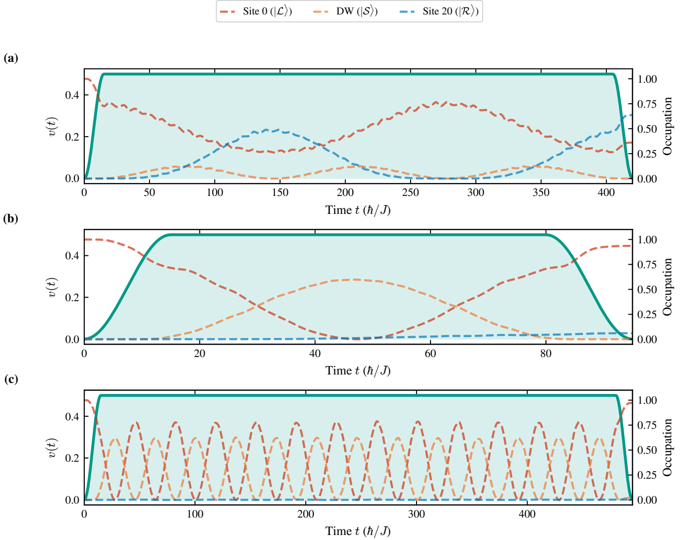
FIG. 7. Transfer dynamics for asymmetric domain wall configurations ( L = 21 ). The fidelity degrades dramatically as the domain wall moves away from the chain center.
