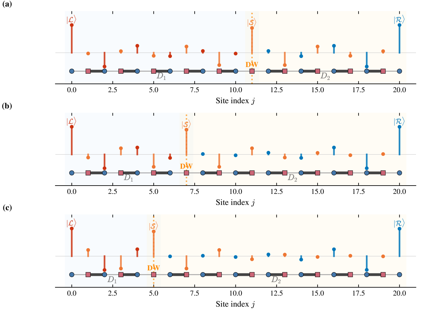
FIG. 5. Spatial profiles of the three protected states for different domain wall positions in an L = 21 chain. Top to bottom: j_{\text{DW}} = 11 (quasi-center), j_{\text{DW}} = 7 (one-third), j_{\text{DW}} = 5 (one-quarter). The exponential localization and sublattice polarization are preserved in all cases.
