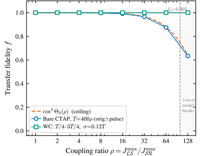
FIG. 15. Transfer fidelity versus the peak-coupling ratio \rho = J_{\text{max}}^L / J_{\text{SR}}^{\text{max}} for the effective three-level system, identifying the residual ceiling as a pulse boundary-condition effect. At the original pulse separation, the converged bare-CTAP fidelity (blue, T = 400\rho ) tracks the analytic ceiling \cos^2 \Theta_0(\rho) [dashed; Eq. (29)]. Re-conditioned pulses (teal; peaks at T/4 and 3T/4 , \sigma = 0.12T ) drive \Theta_0 \rightarrow 0 and keep f \approx 1 across the whole range. Beyond \rho \gtrsim 10^2 (shaded) the protected gap of the real chain closes and the three-level description ceases to apply. Dotted line: f_0 = 0.995 .
