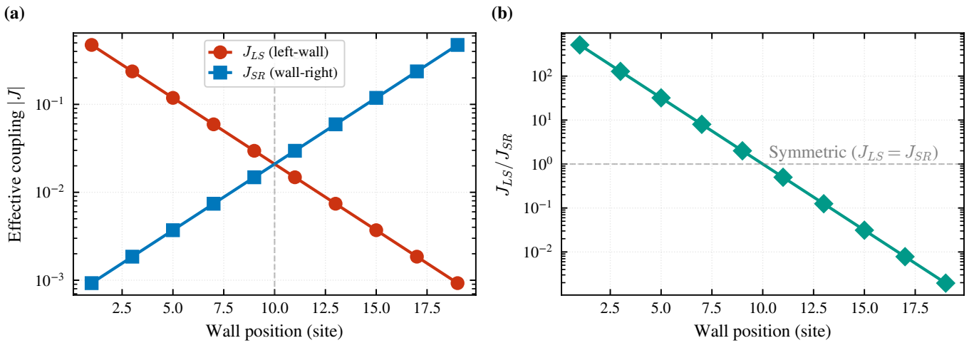
FIG. 6. Effective couplings J_{\mathcal{L}\mathcal{S}} (left-soliton) and J_{\mathcal{S}\mathcal{R}} (soliton-right) as a function of the domain wall position for L = 21 . The coupling asymmetry grows exponentially with the displacement from the chain center, consistent with Eq. (12).
