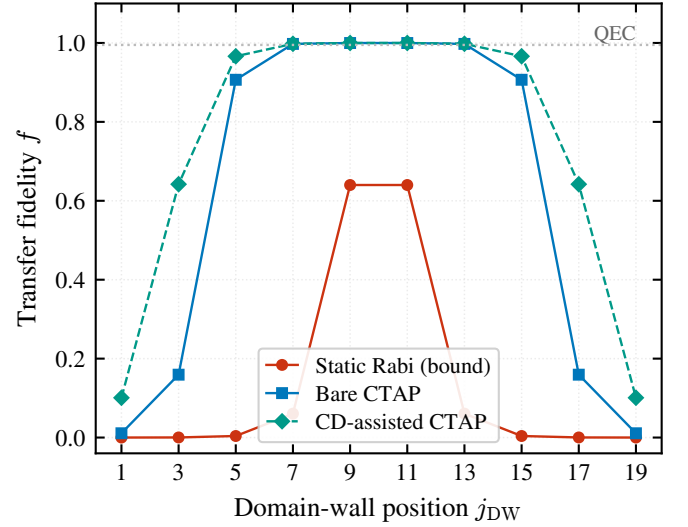
FIG. 14. Transfer fidelity versus domain-wall position j_{\text{DW}} for L = 21 ( v = 0.5 , w = 1.0 ), obtained by numerical integration of the effective three-level Hamiltonian (21). The static Rabi protocol (red circles) peaks at f \approx 0.64 near the quasi-center and collapses to f \lesssim 0.004 for j_{\text{DW}} \leq 5 . Bare CTAP (blue squares), driven by the counter-intuitive Gaussian pulses [Eqs. (25)–(26)], sustains f > 0.99 over a broad central region and degrades only for extreme asymmetry. CD-assisted CTAP (teal diamonds) widens the high-fidelity plateau by suppressing the residual nonadiabatic error. The dotted line marks the fault-tolerance threshold f_0 = 0.995 .
