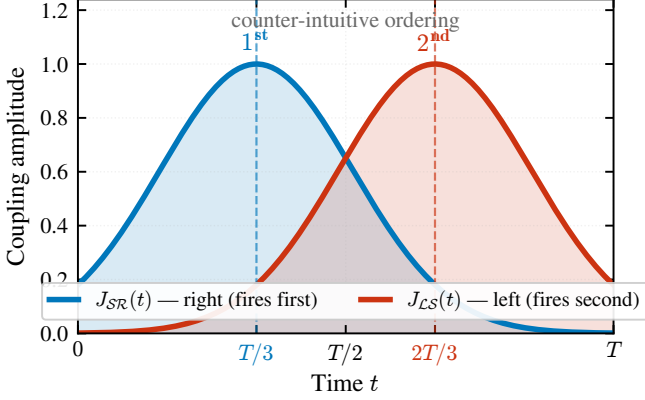
FIG. 13. (a) Counter-intuitive CTAP pulse sequence. The right-domain coupling J_{SR}(t) (blue) fires before the left-domain coupling J_{LS}(t) (red), adiabatically rotating the mixing angle \Theta(t) from 0 to \pi/2 over the transfer time T . (b) Population dynamics of the effective three-level system under the CTAP protocol ( T = 300 , \sigma = 0.18T , J_{\max} = 1 ). Starting from |\mathcal{L}\rangle (red), population is transferred to |\mathcal{R}\rangle (blue) with final fidelity f = 0.9999 . The soliton state |\mathcal{S}\rangle (gold, dashed) remains at zero throughout (lower panel, log scale)—the hallmark of dark-state transfer via the topological zero mode.
