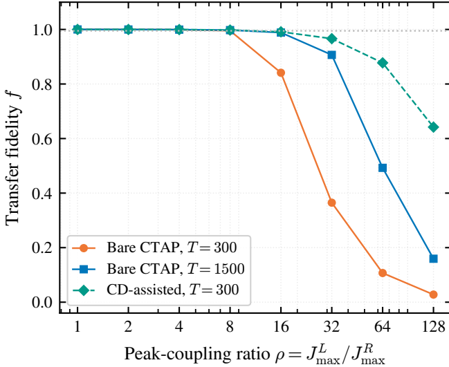
FIG. 15. Transfer fidelity as a function of the peak-coupling ratio \rho = J_{\max}^L / J_{\max}^R for the effective three-level system. Bare CTAP at T = 300 (orange) and T = 1500 (blue), and CD-assisted CTAP at T = 300 (teal). High fidelity is maintained up to \rho \approx 16 ; beyond \rho \sim 10^2 the protected gap closes and the dark-state mechanism ceases to apply. Dotted line: f_0 = 0.995 .
