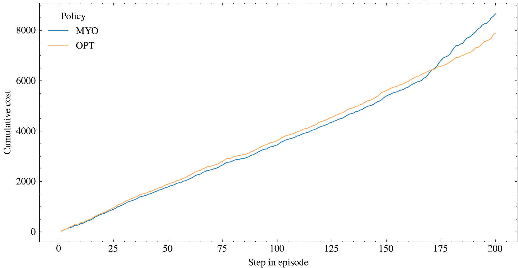
Cumulative cost over episode - instance 10001 (5 facilities, 200 orders, uneven capacity)
