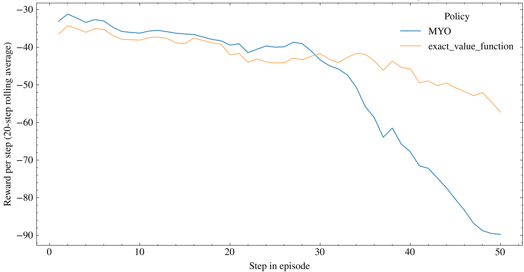
Reward rate over episode - instance 10001 (5 facilities, 50 orders, uneven capacity)
