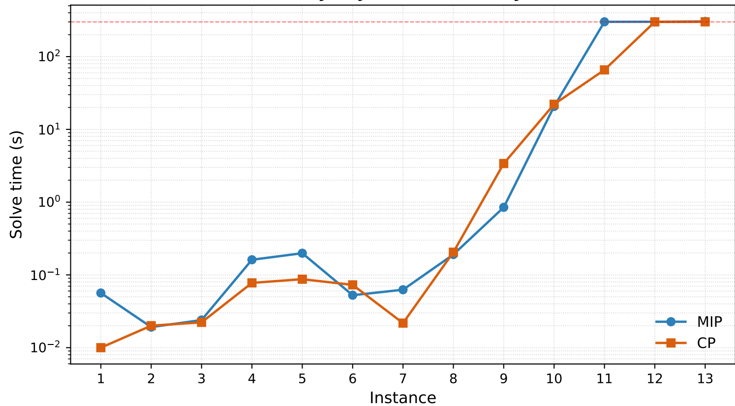
MIP vs CP — Solve Time Penalty objective, 2 runway(s)
