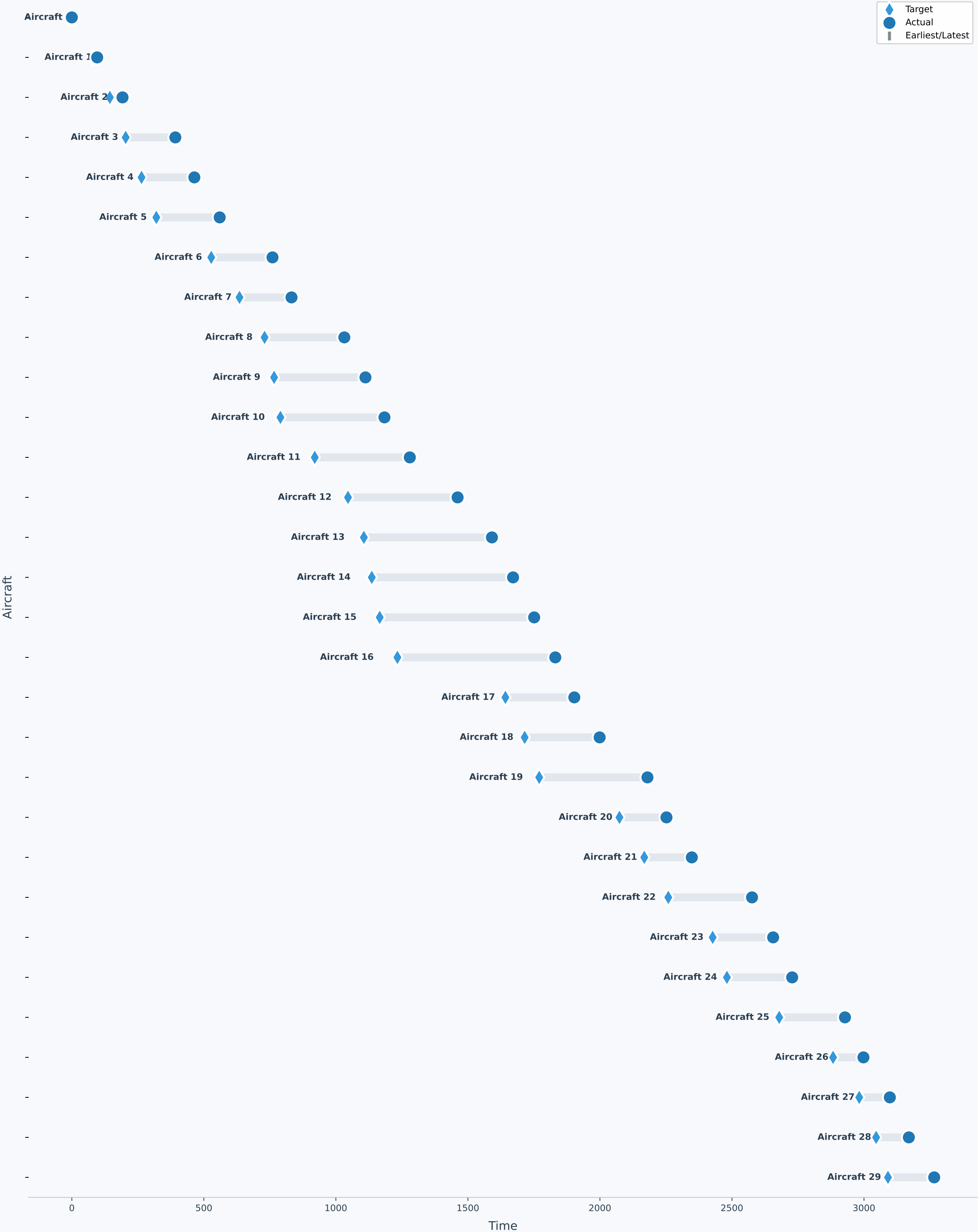
Schedule Details -- Instance 6 | 1 Runways | makespan | MIP
