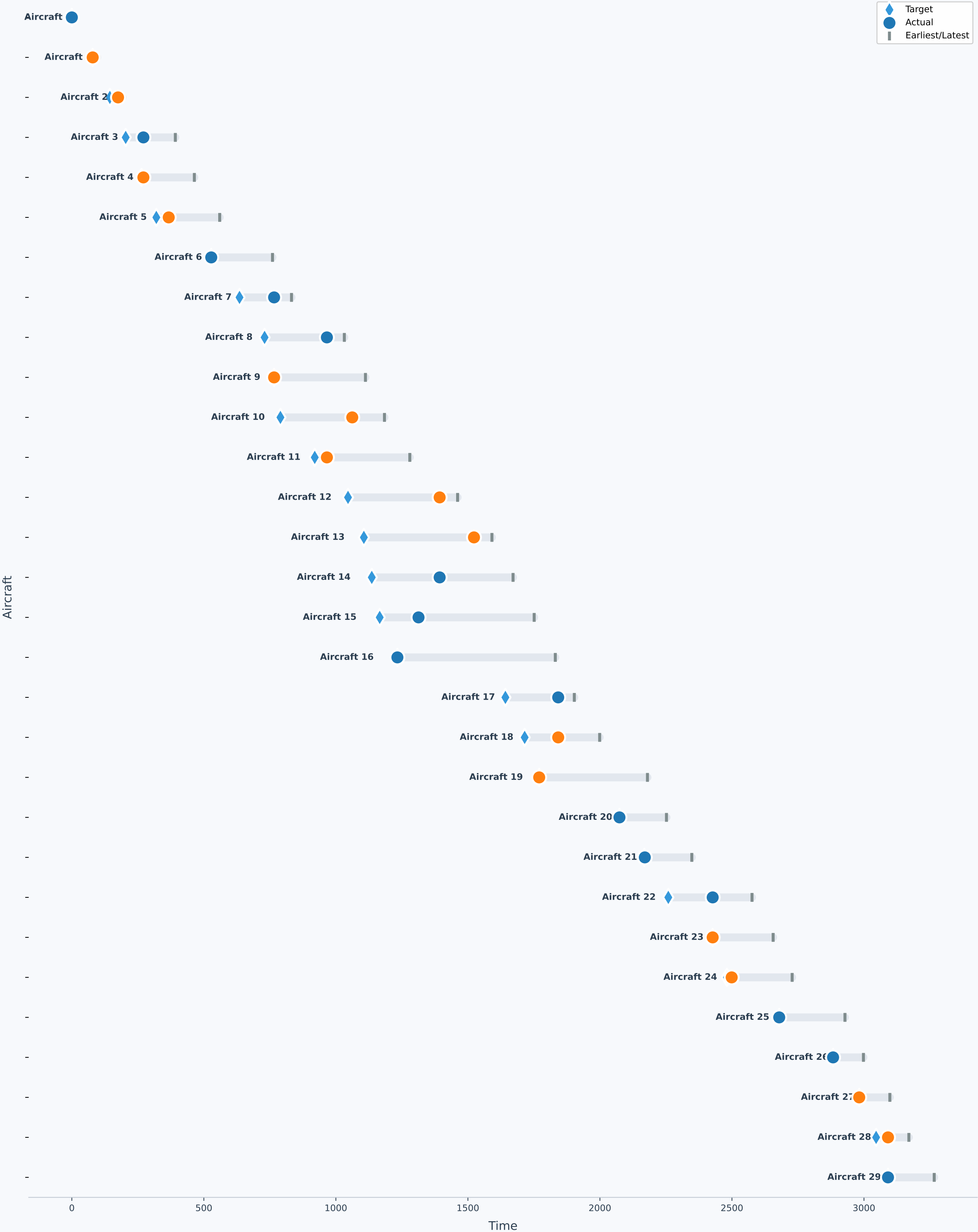
Schedule Details -- Instance 6 | 2 Runways | makespan | MIP
