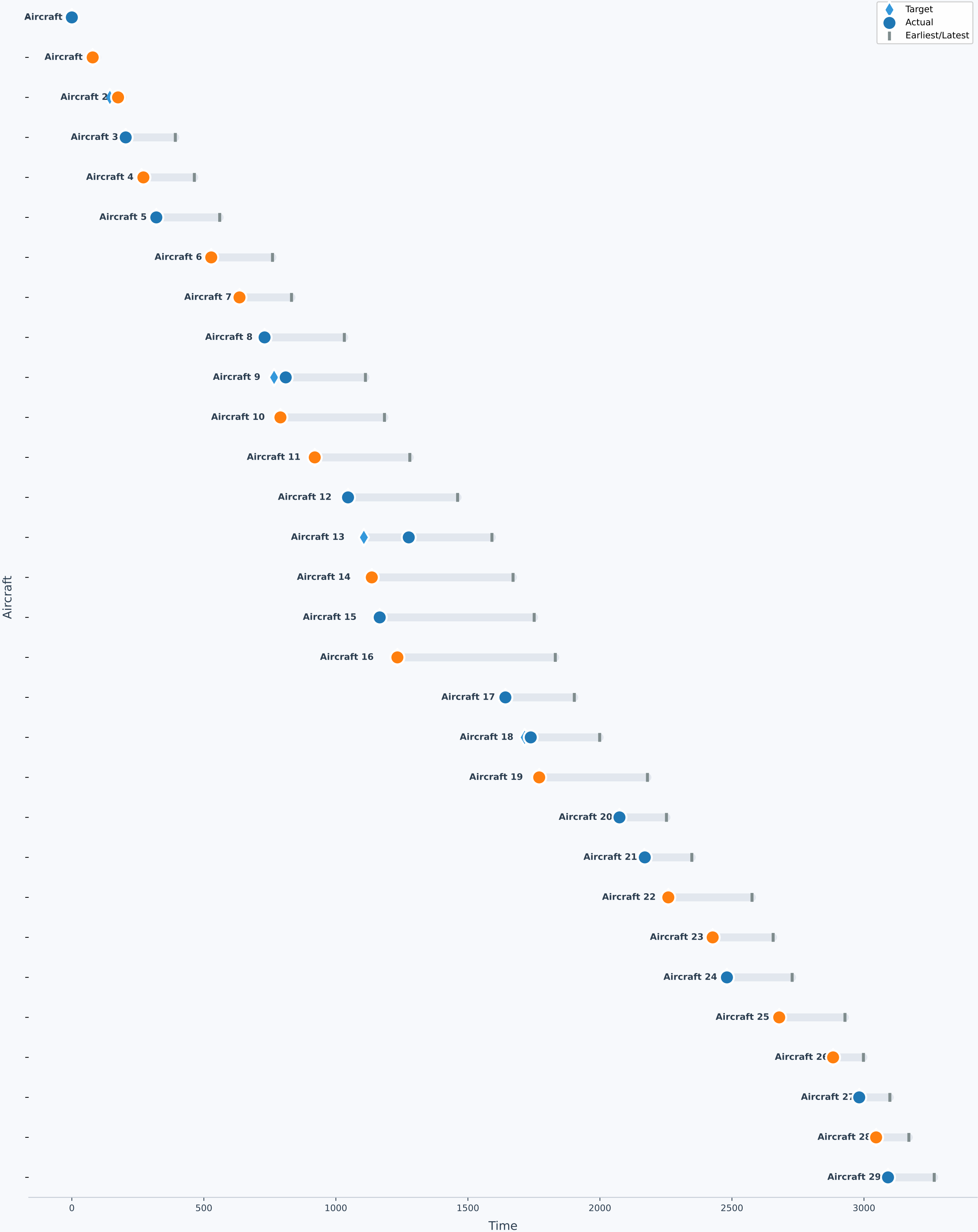
Schedule Details -- Instance 6 | 2 Runways | penalty | MIP
